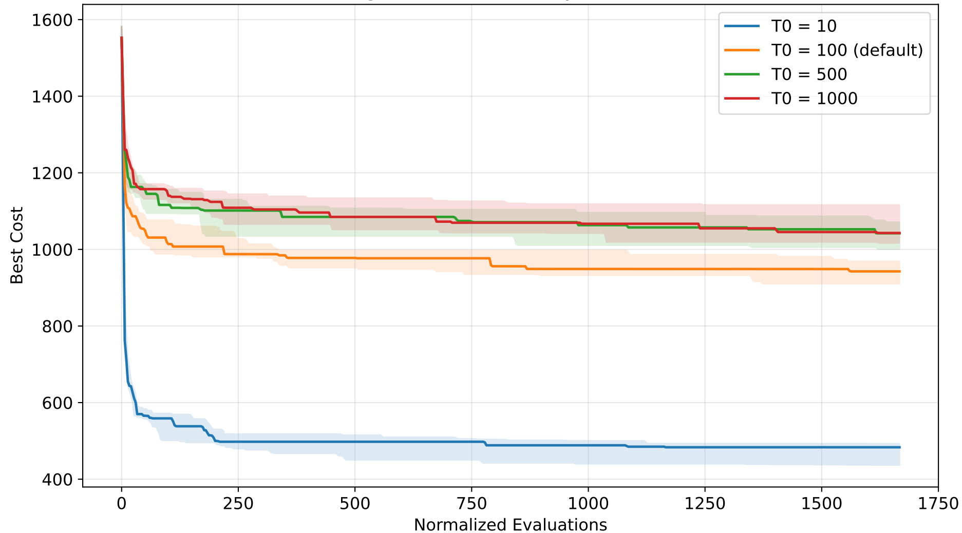
SA convergence - T0 sensitivity (TSP, normalized)
