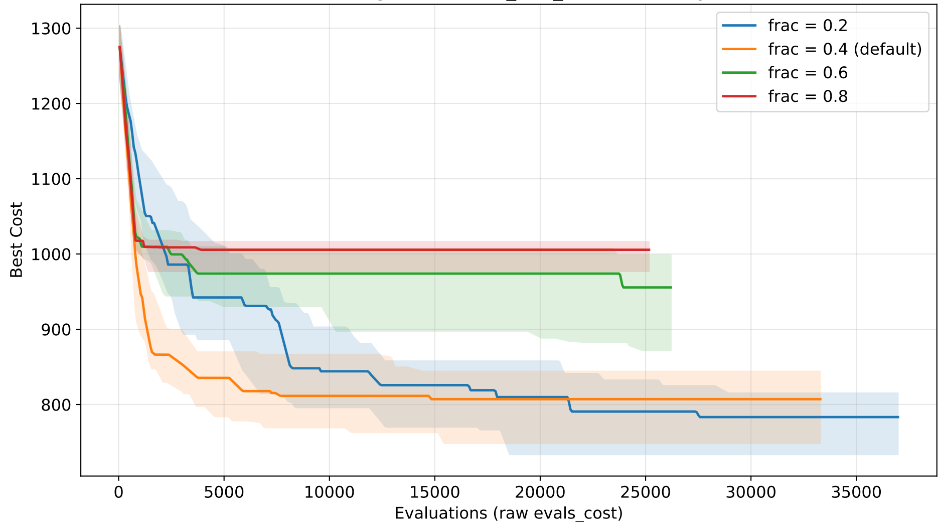
TLBO convergence - move_frac_max sensitivity (TSP)
