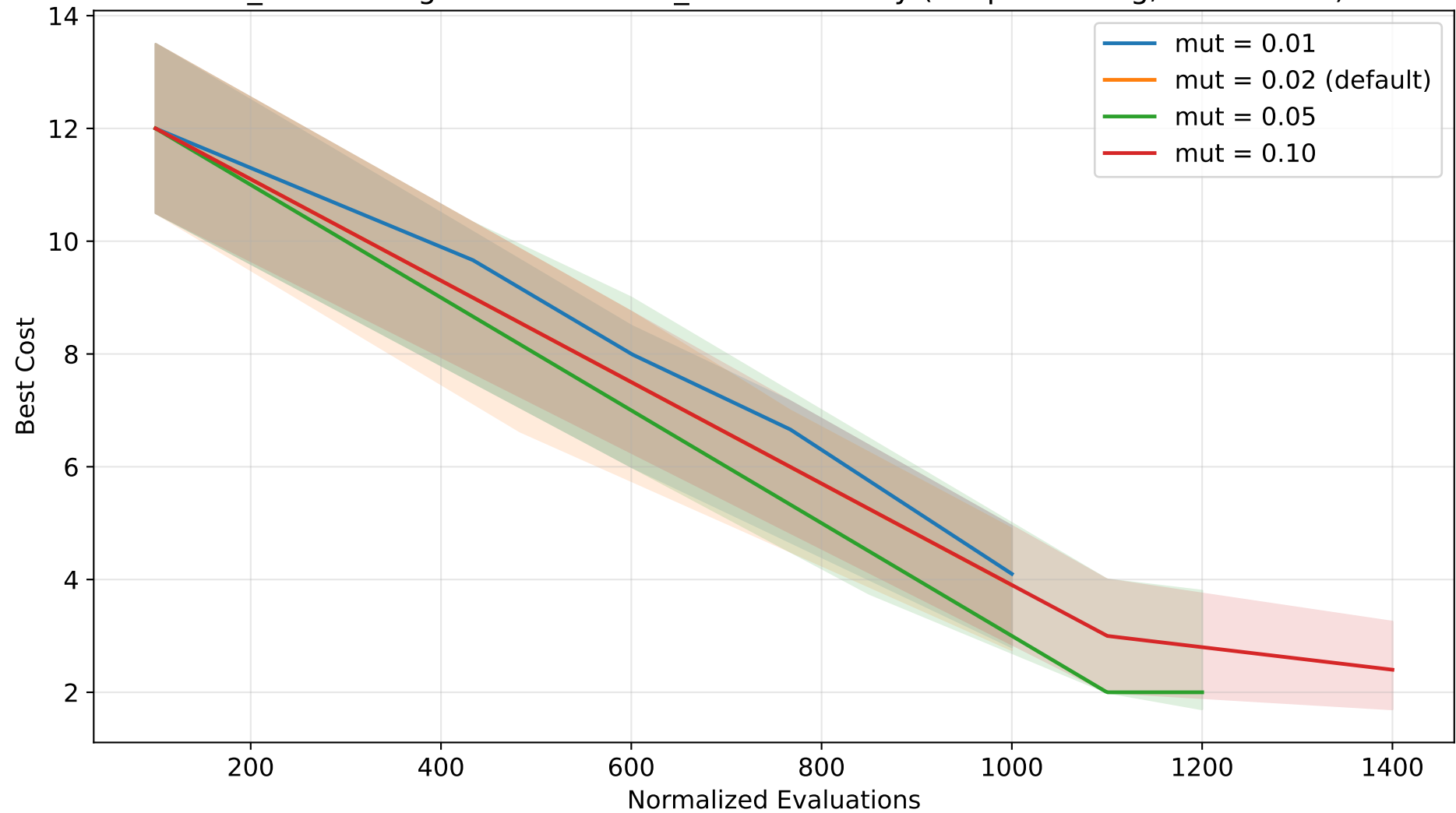
GA_GC convergence - mutation_rate sensitivity (GraphColoring, normalized)
