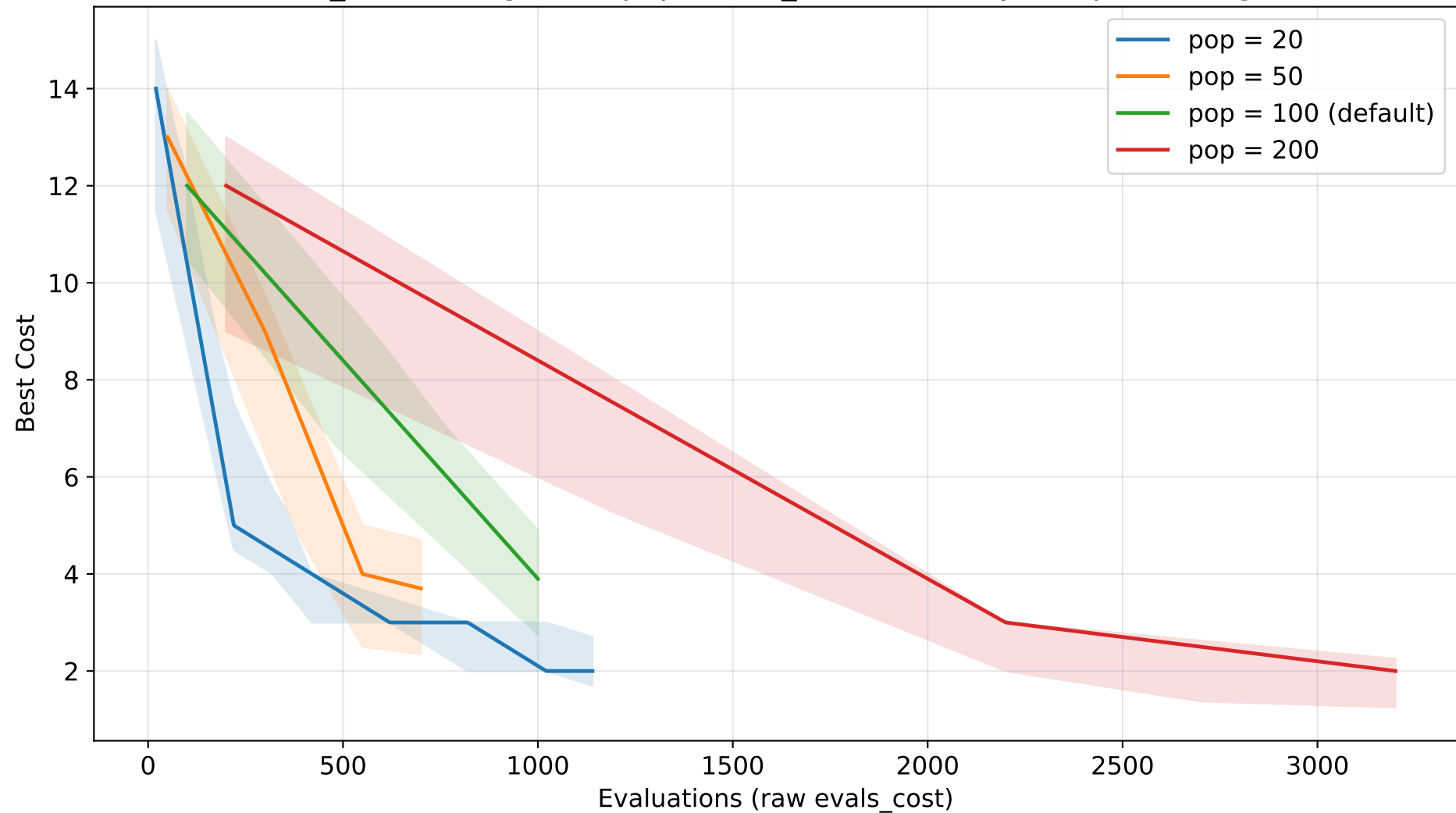
GA_GC convergence - population_size sensitivity (GraphColoring)
