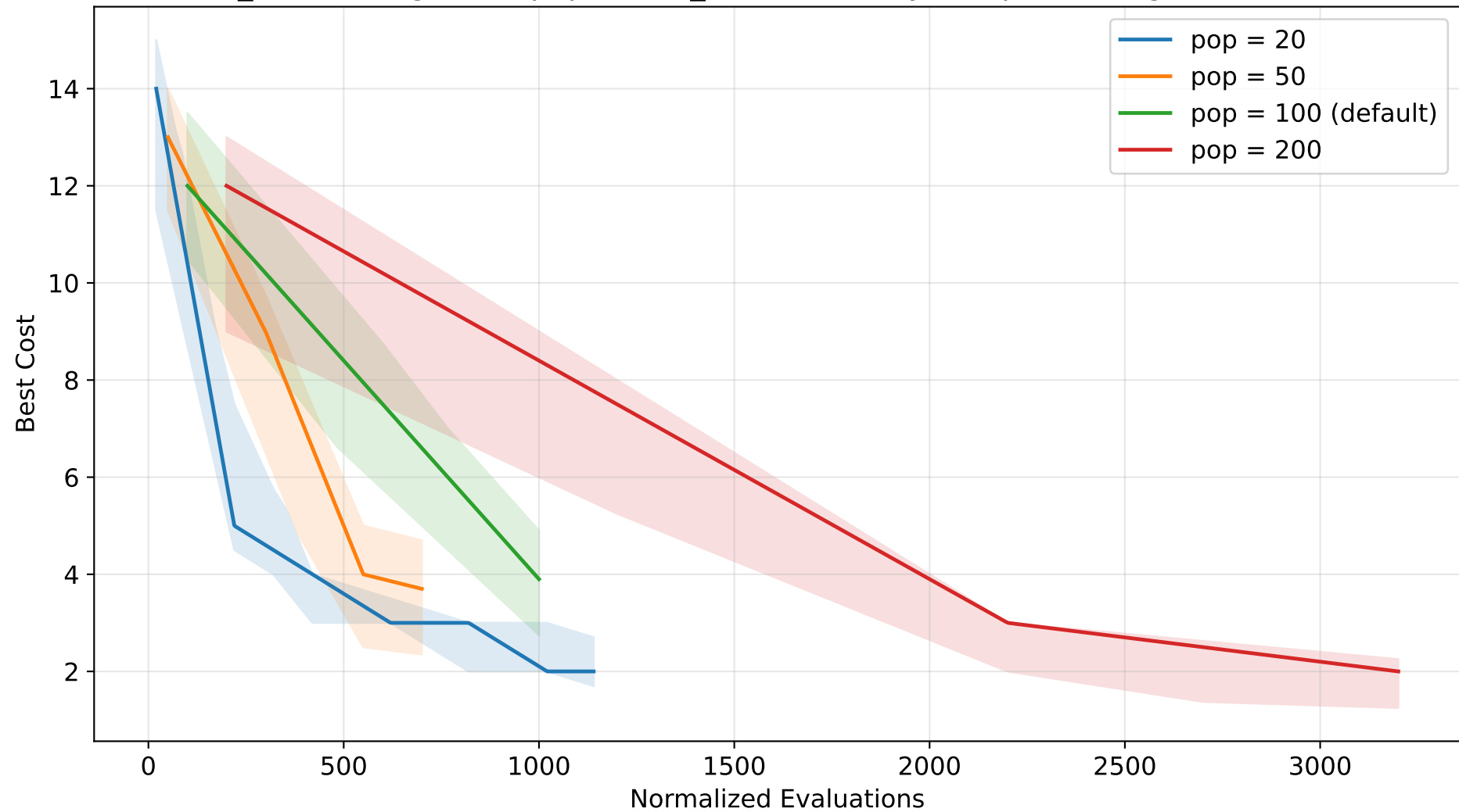
GA_GC convergence - population_size sensitivity (GraphColoring, normalized)
