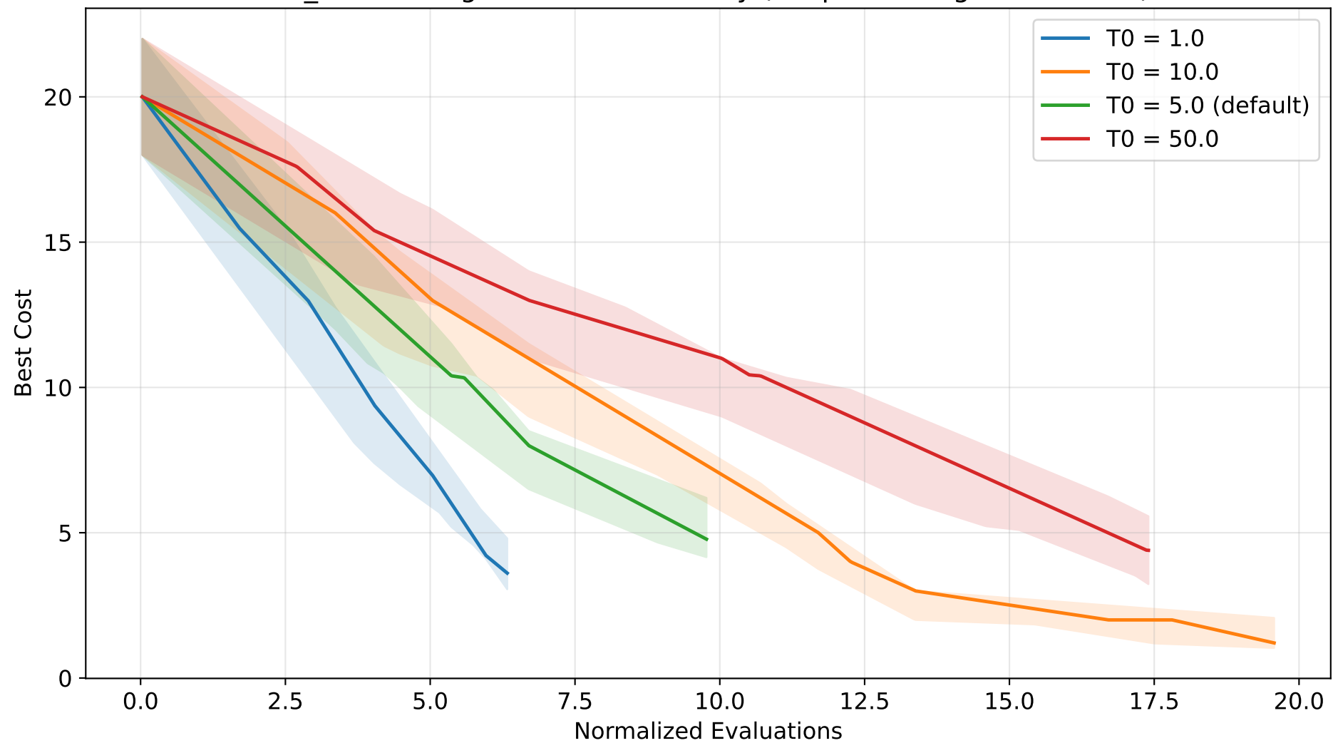
SA_GC convergence - T0 sensitivity (GraphColoring, normalized)
