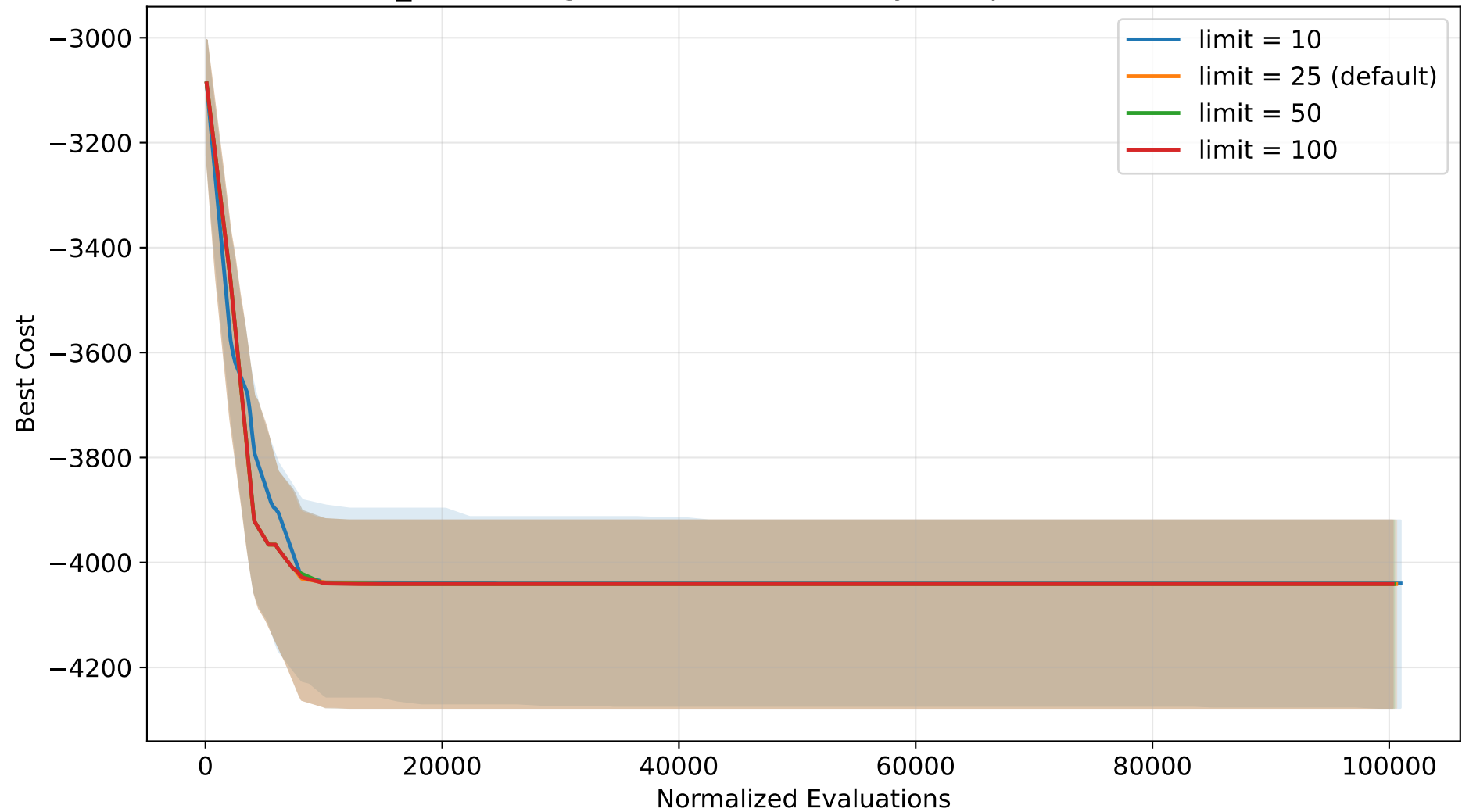
ABC_KP convergence - limit sensitivity (Knapsack, normalized)
