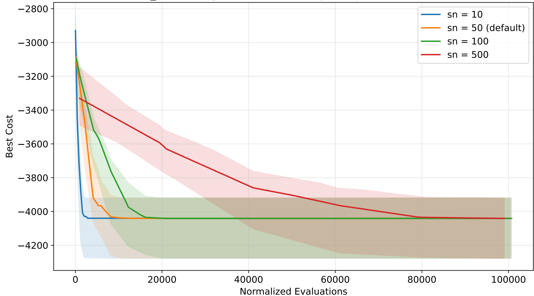
ABC_KP convergence - sn sensitivity (Knapsack, normalized)
