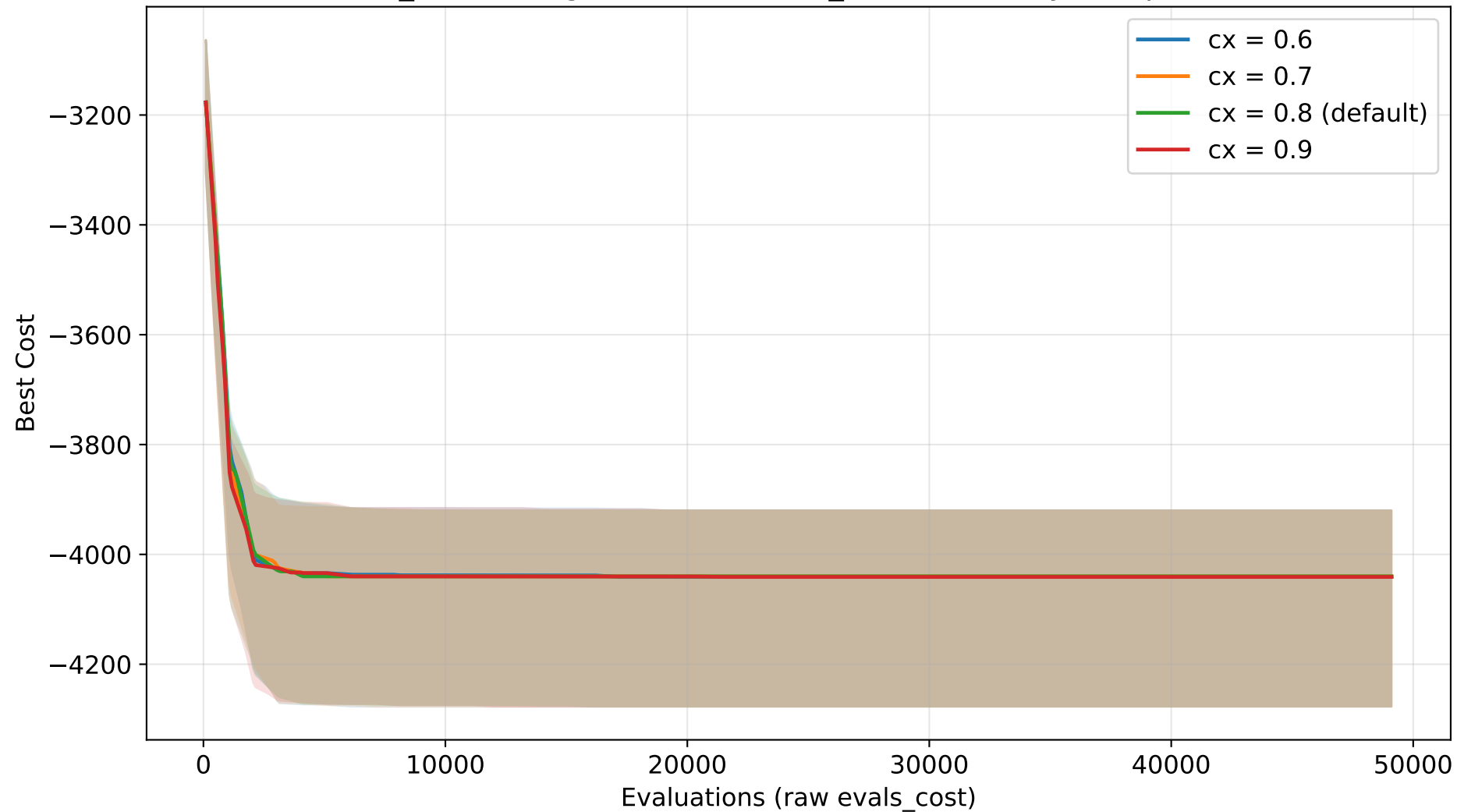
GA_KP convergence - crossover_rate sensitivity (Knapsack)
