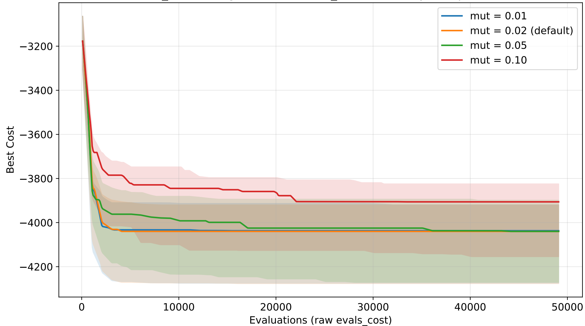
GA_KP convergence - mutation_rate sensitivity (Knapsack)
