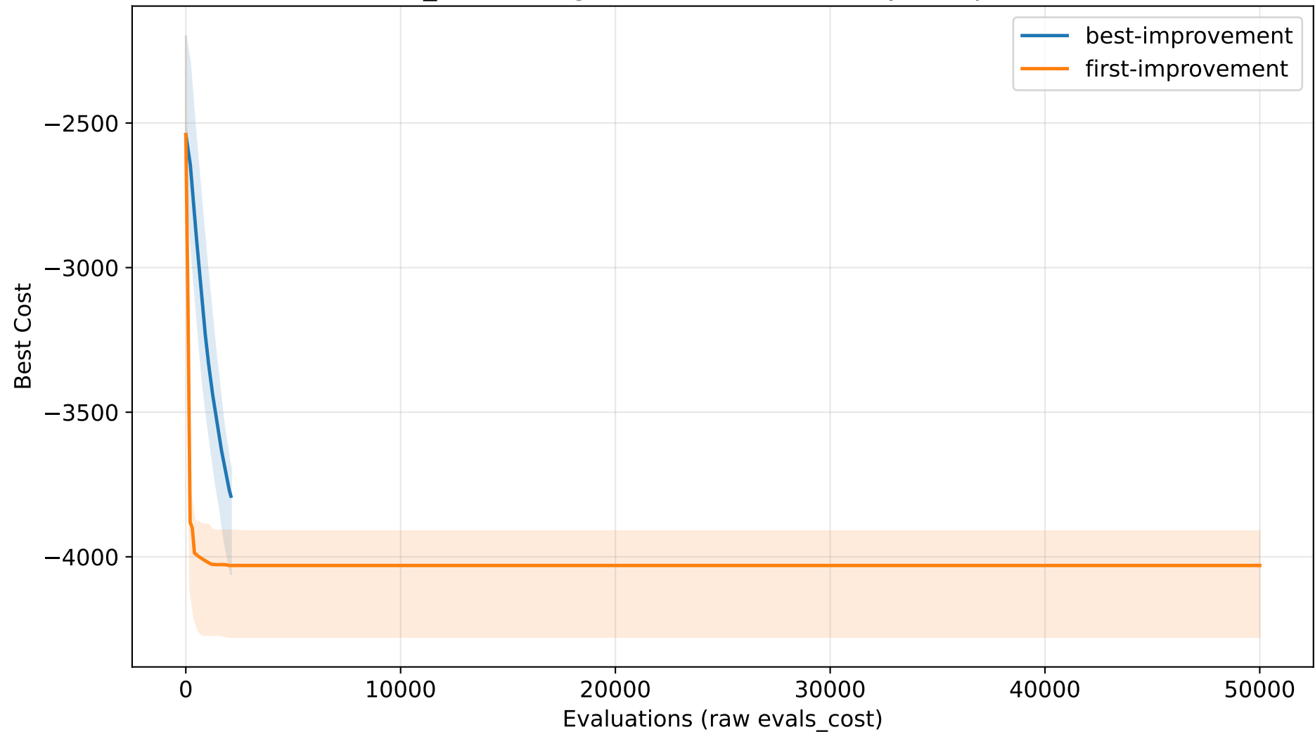
HC_KP convergence - mode sensitivity (Knapsack)
