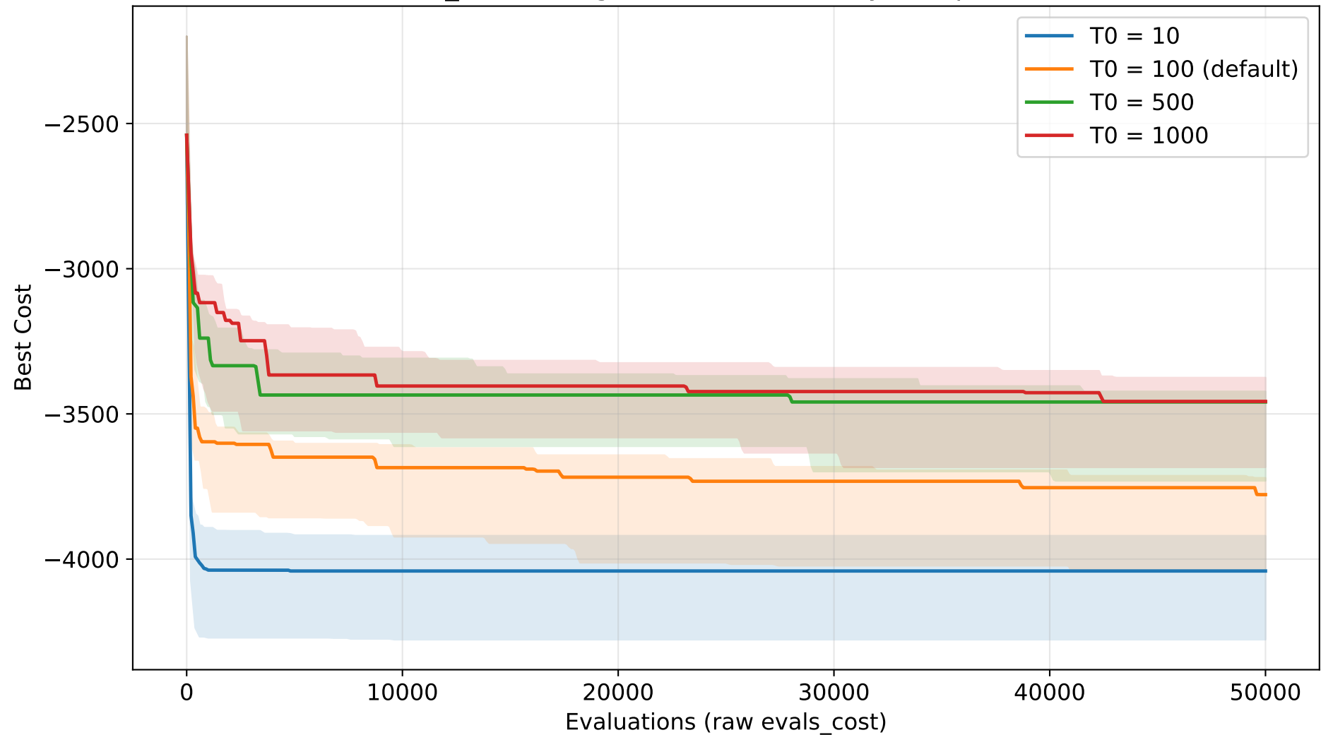
SA_KP convergence - T0 sensitivity (Knapsack)
