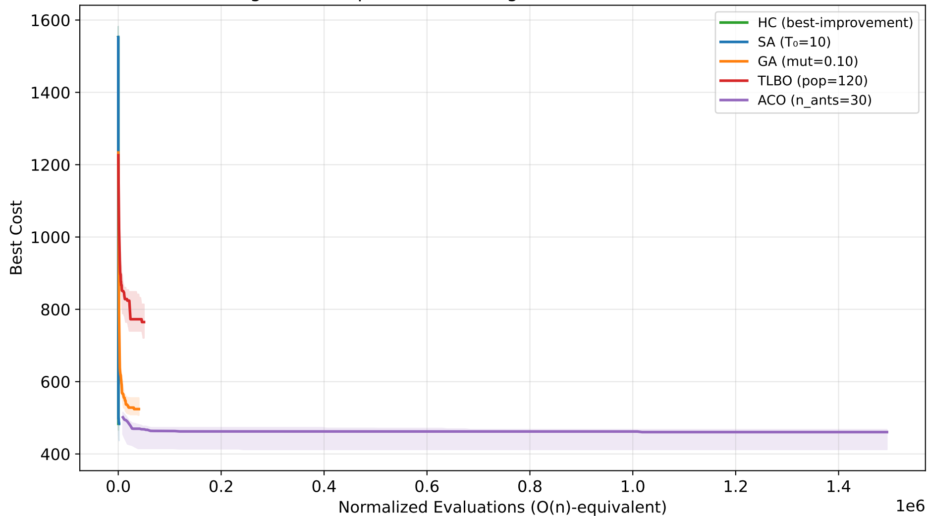
Convergence Comparison — All Algorithms (TSP n=30, normalized)
