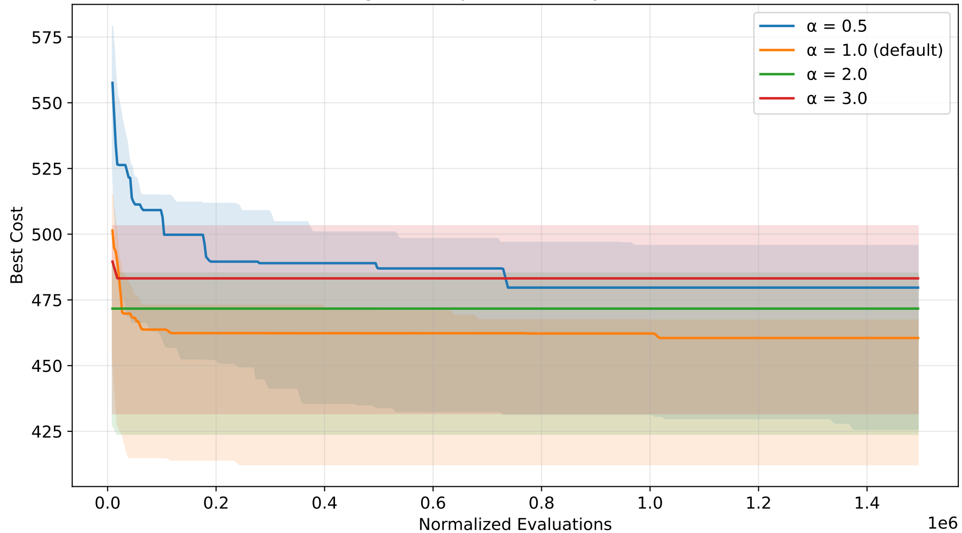
ACO convergence - alpha sensitivity (TSP, normalized)
