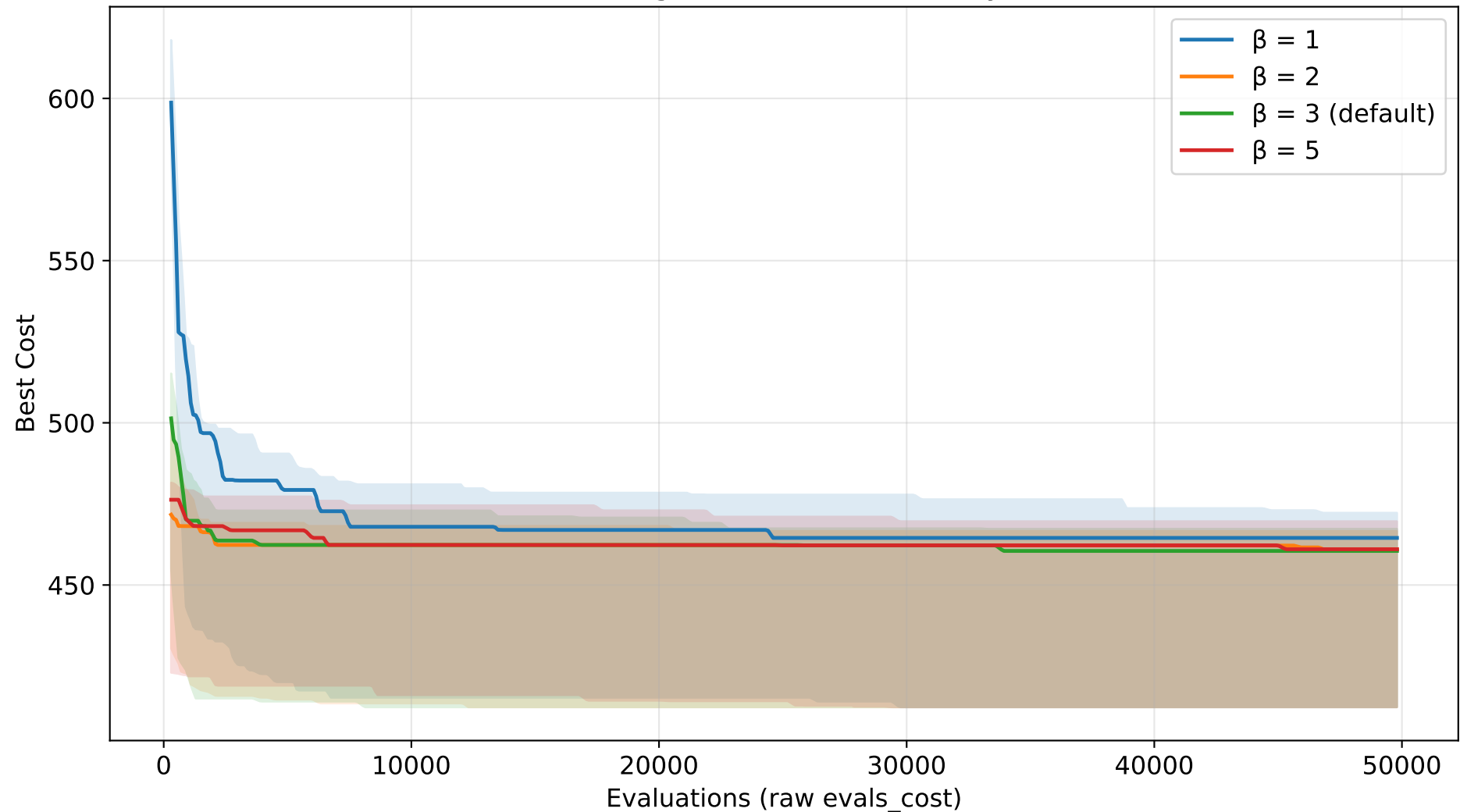
ACO convergence - beta sensitivity (TSP)
