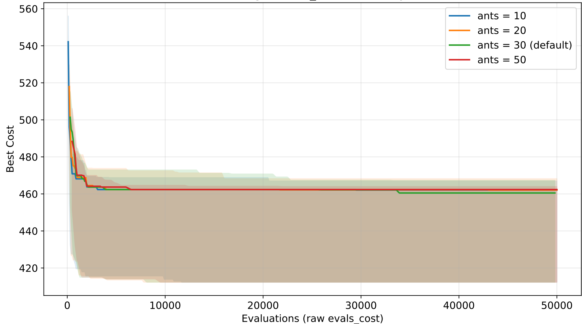
ACO convergence - n_ants sensitivity (TSP)
