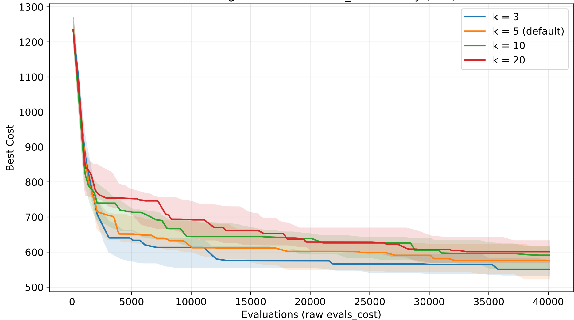
GA convergence - tournament_k sensitivity (TSP)
