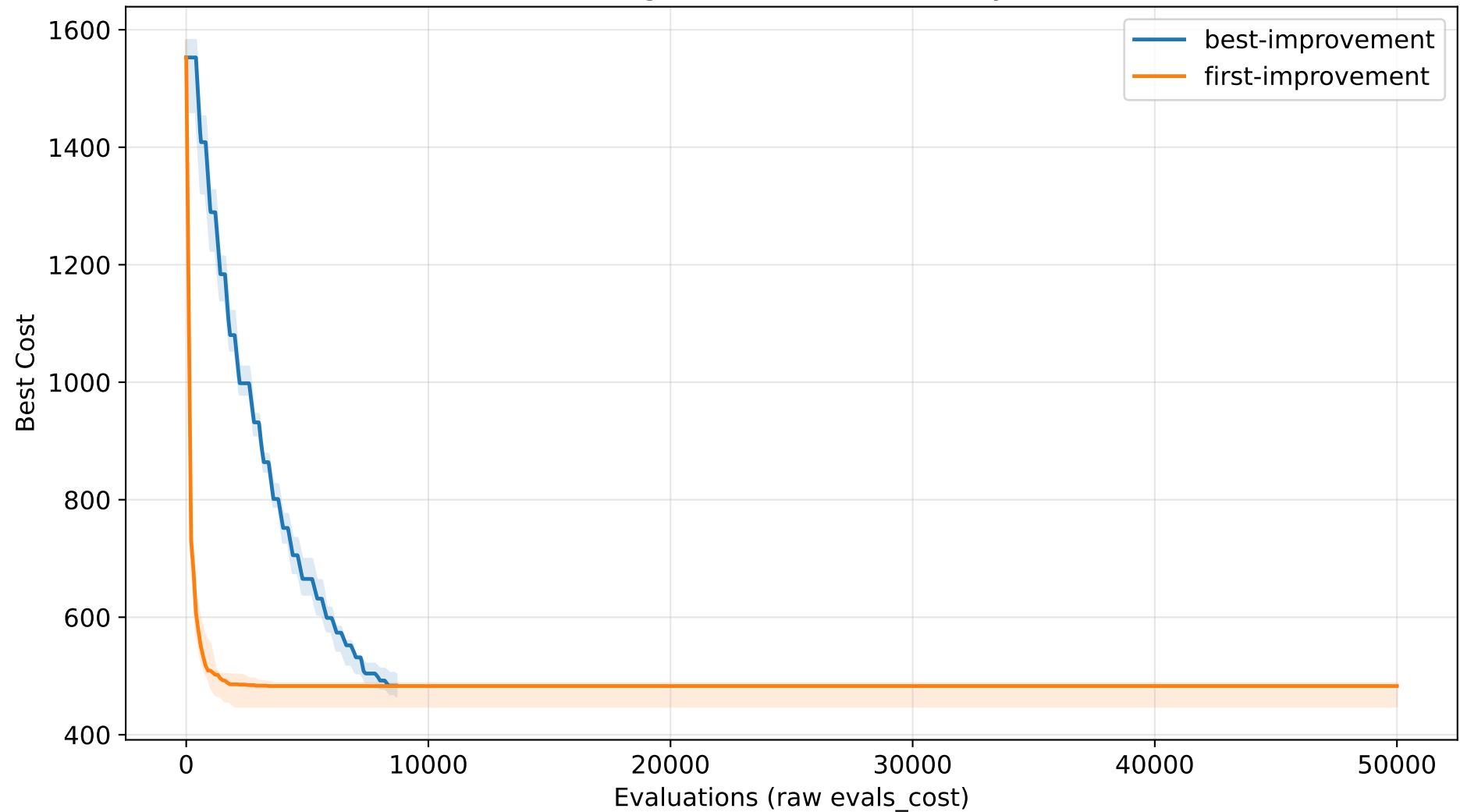
HC convergence - mode sensitivity (TSP)
