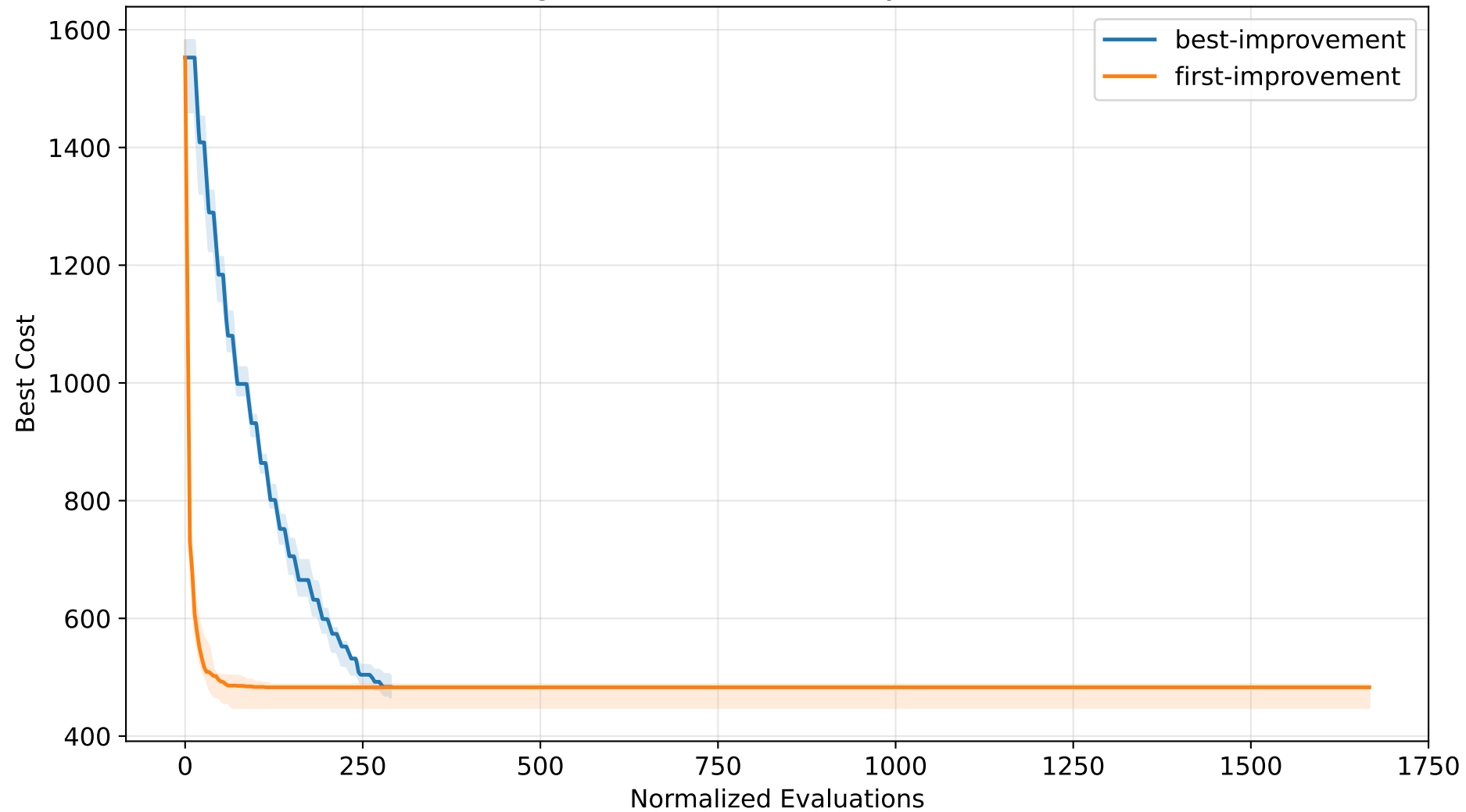
HC convergence - mode sensitivity (TSP, normalized)
