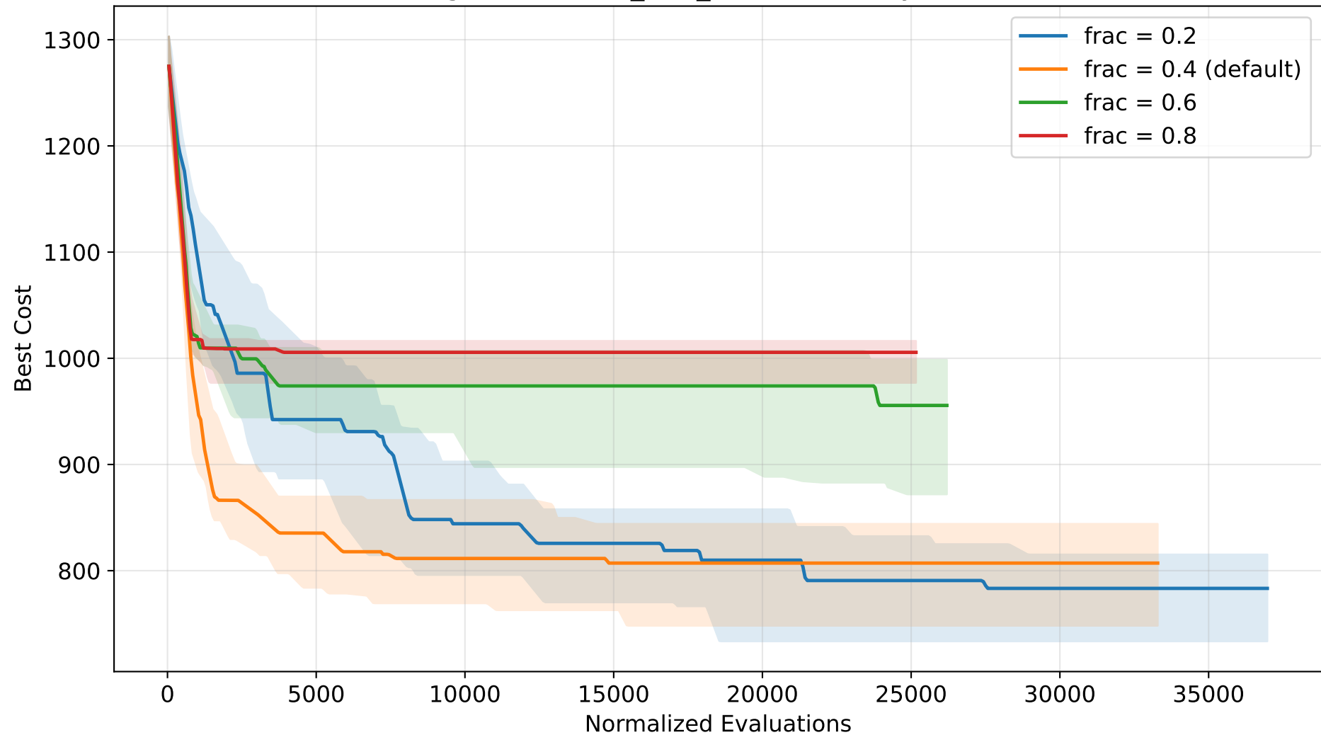
TLBO convergence - move_frac_max sensitivity (TSP, normalized)
