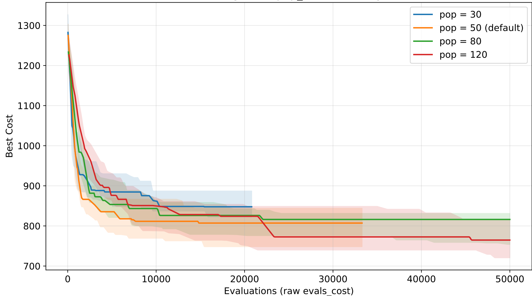
TLBO convergence - pop_size sensitivity (TSP)
