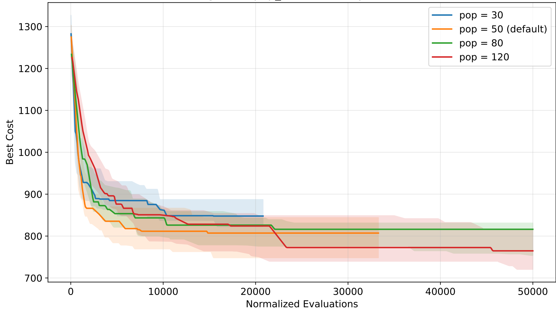
TLBO convergence - pop_size sensitivity (TSP, normalized)
