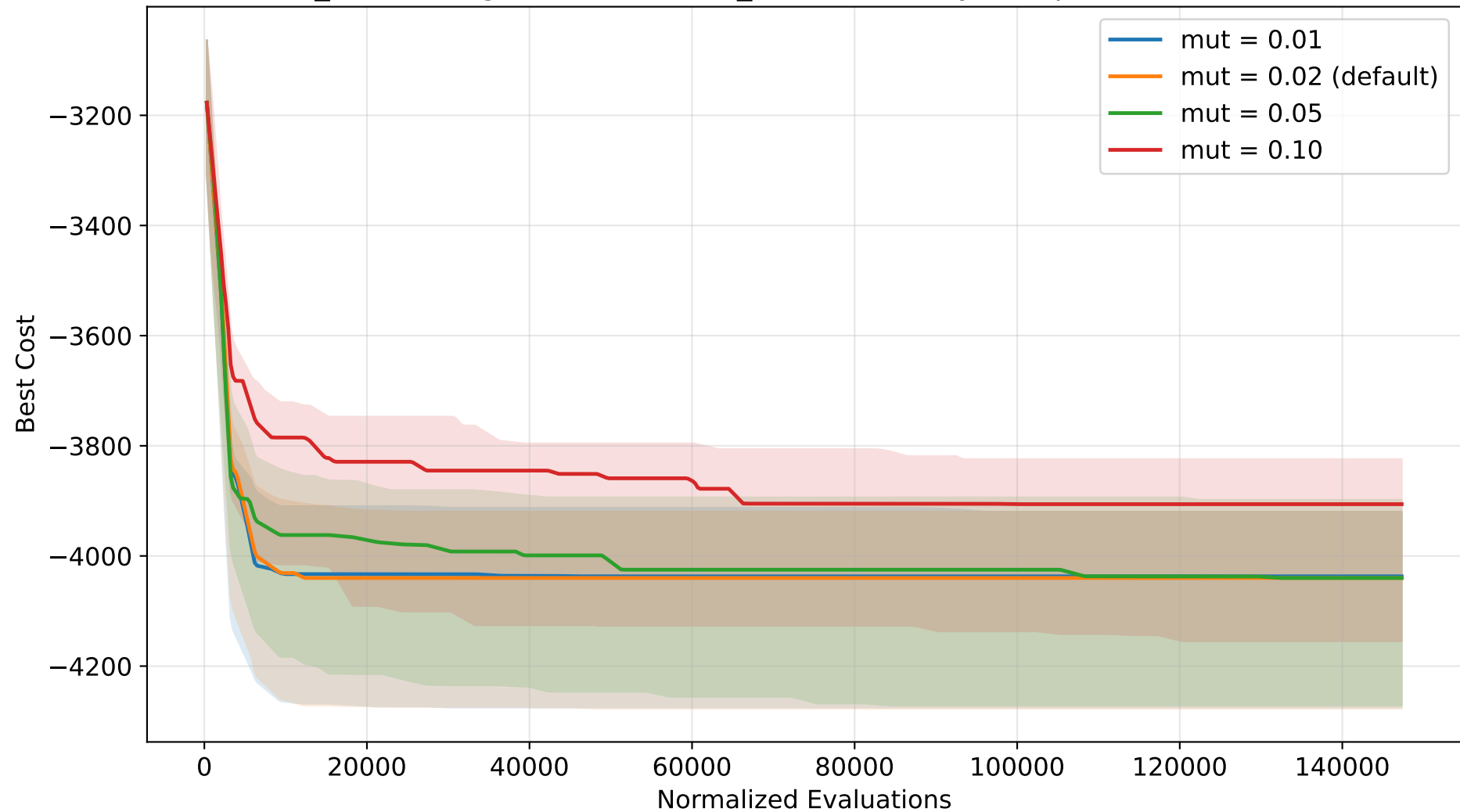
GA_KP convergence - mutation_rate sensitivity (Knapsack, normalized)
