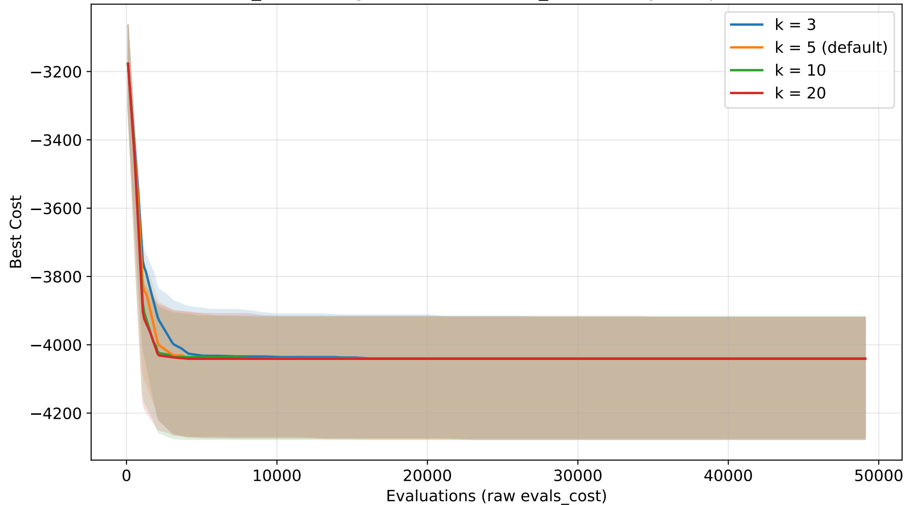
GA_KP convergence - tournament_k sensitivity (Knapsack)
