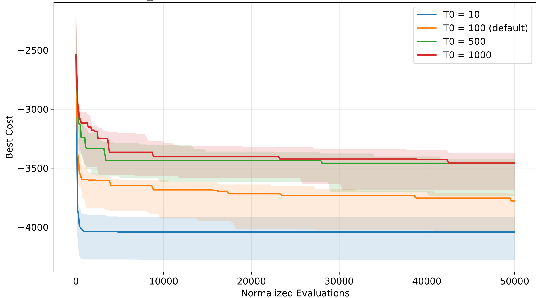
SA_KP convergence - T0 sensitivity (Knapsack, normalized)
