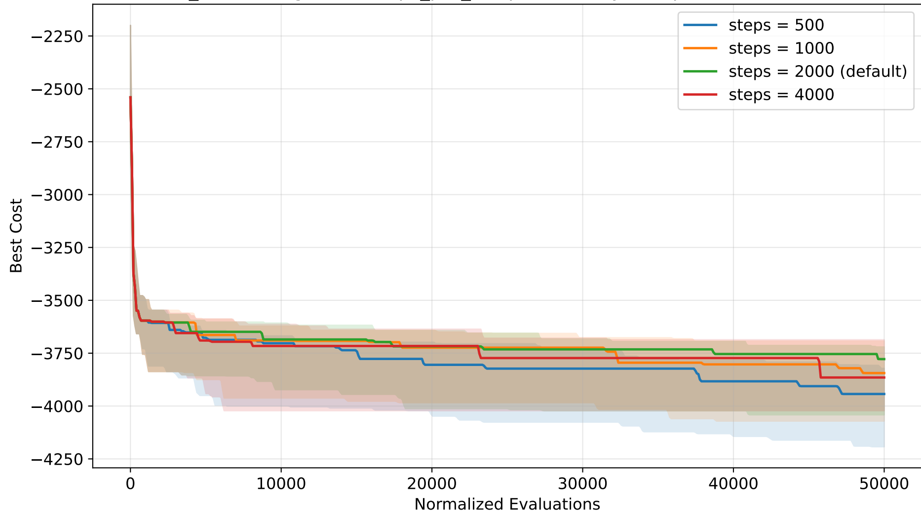
SA_KP convergence - steps_per_temp sensitivity (Knapsack, normalized)
