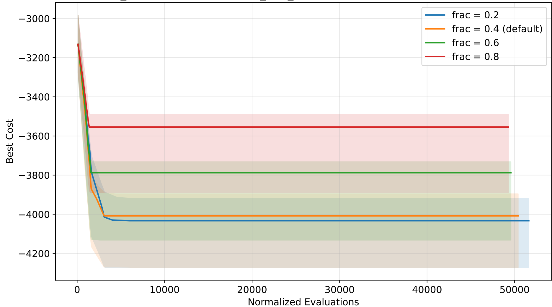
TLBO_KP convergence - move_frac_max sensitivity (Knapsack, normalized)
