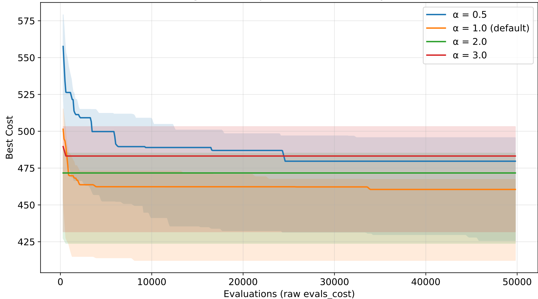
ACO Convergence — \alpha (pheromone) sensitivity (TSP n=30)
