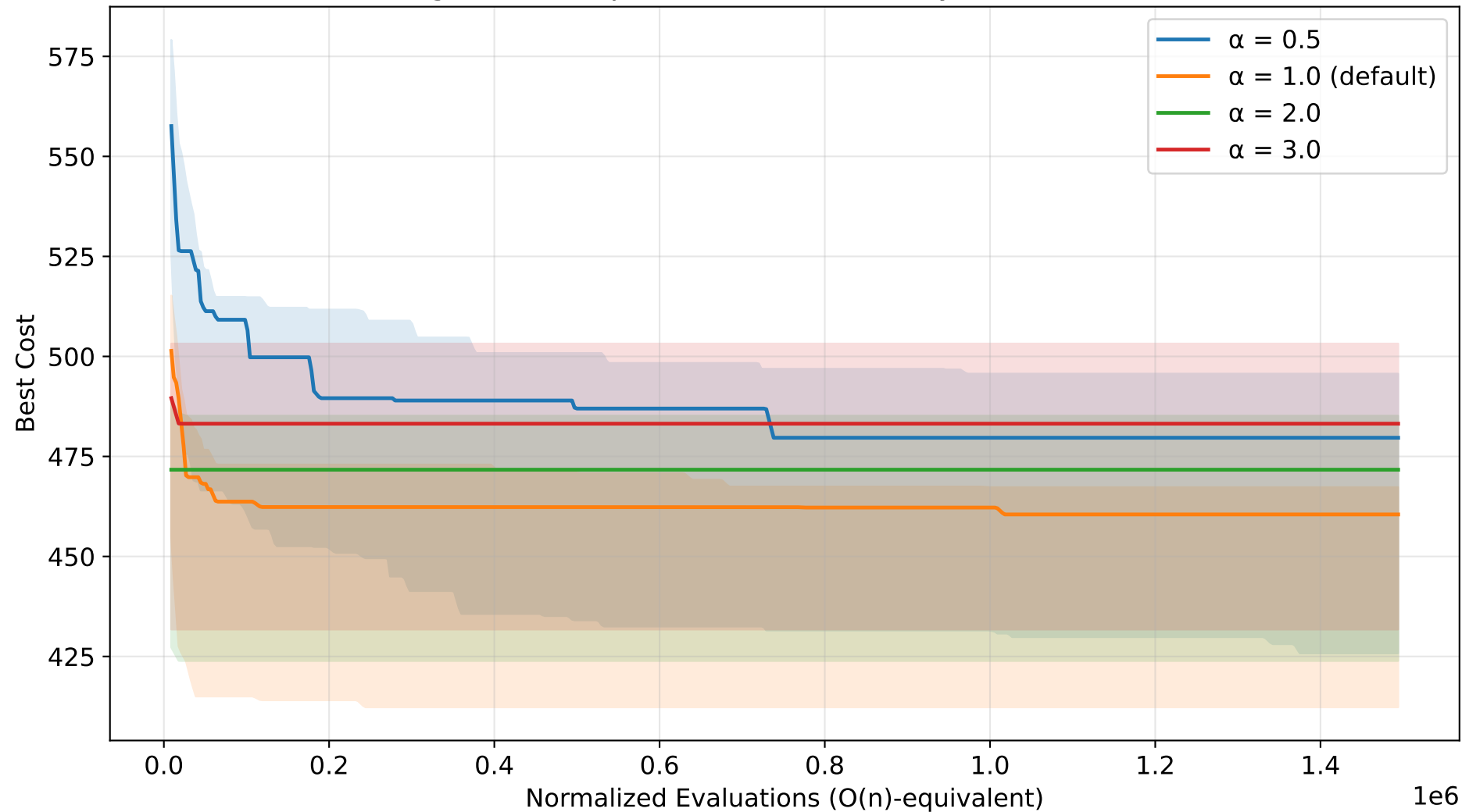
ACO Convergence — \alpha (pheromone) sensitivity (TSP n=30, normalized)
