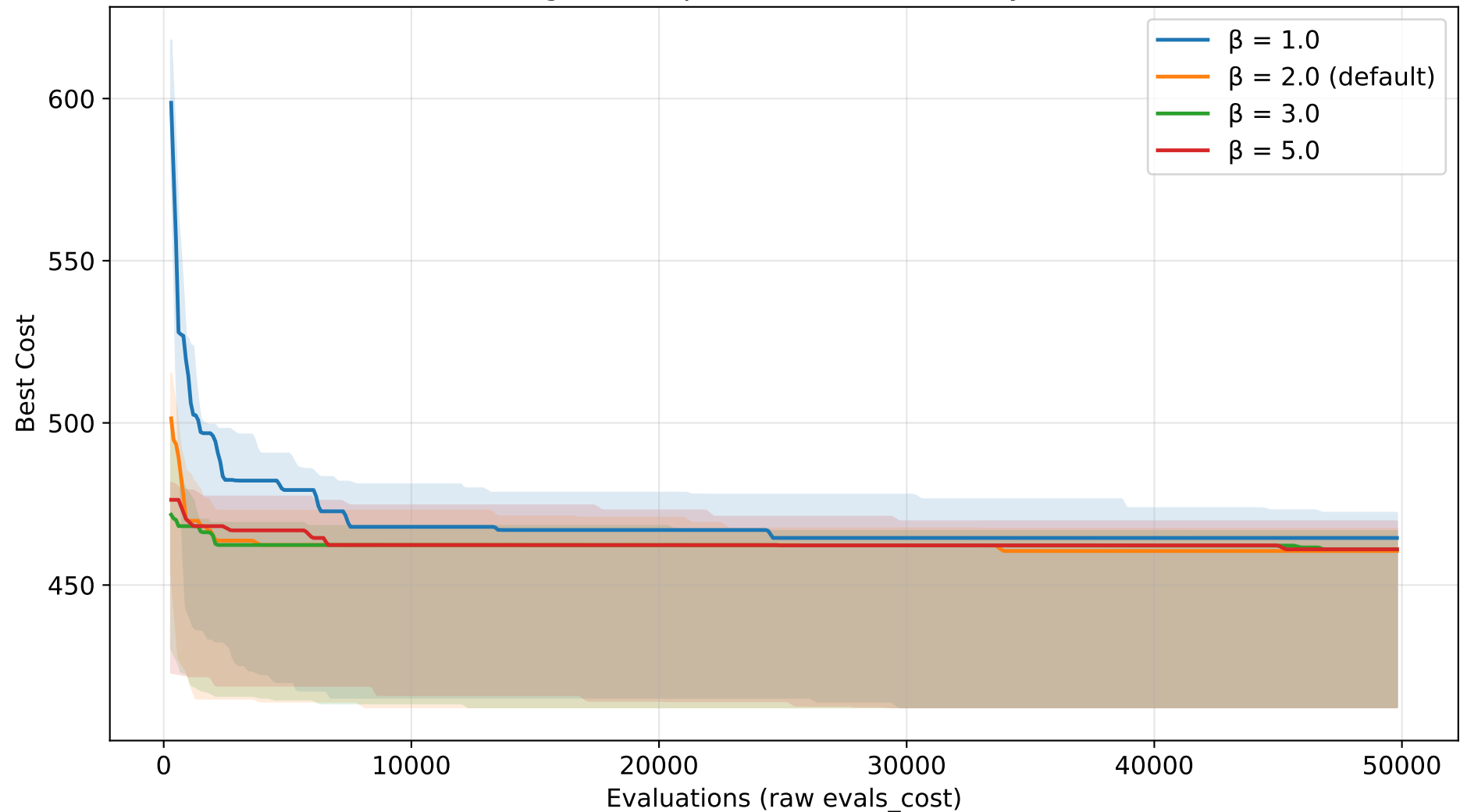
ACO Convergence — \beta (heuristic) sensitivity (TSP n=30)
