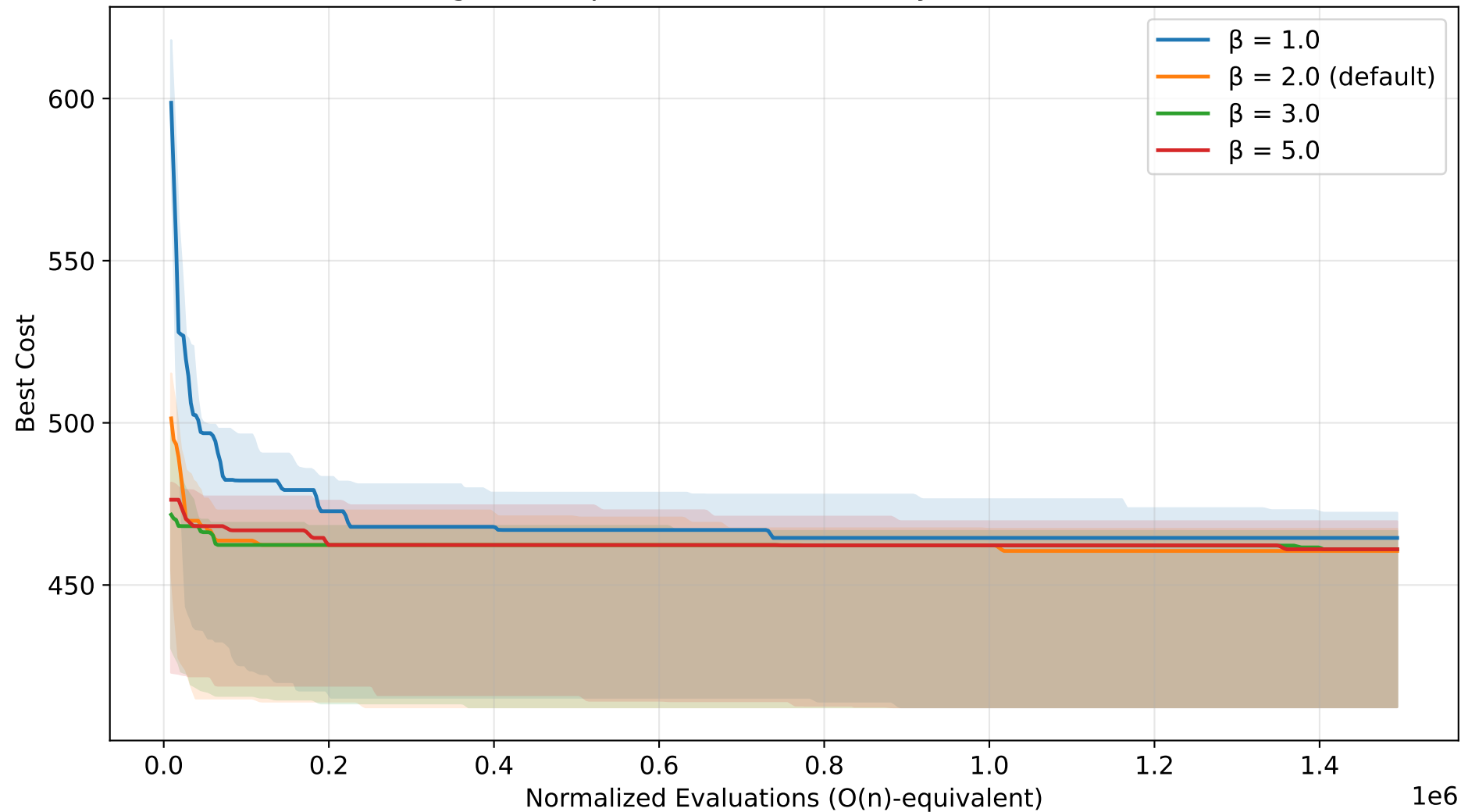
ACO Convergence — \beta (heuristic) sensitivity (TSP n=30, normalized)
