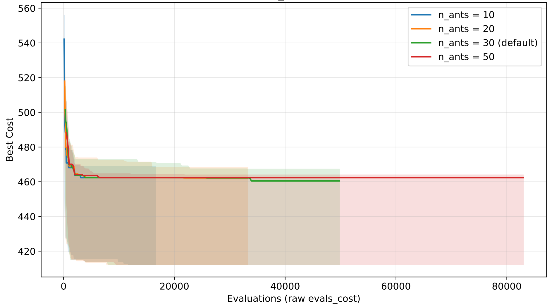
ACO Convergence — n_ants sensitivity (TSP n=30)
