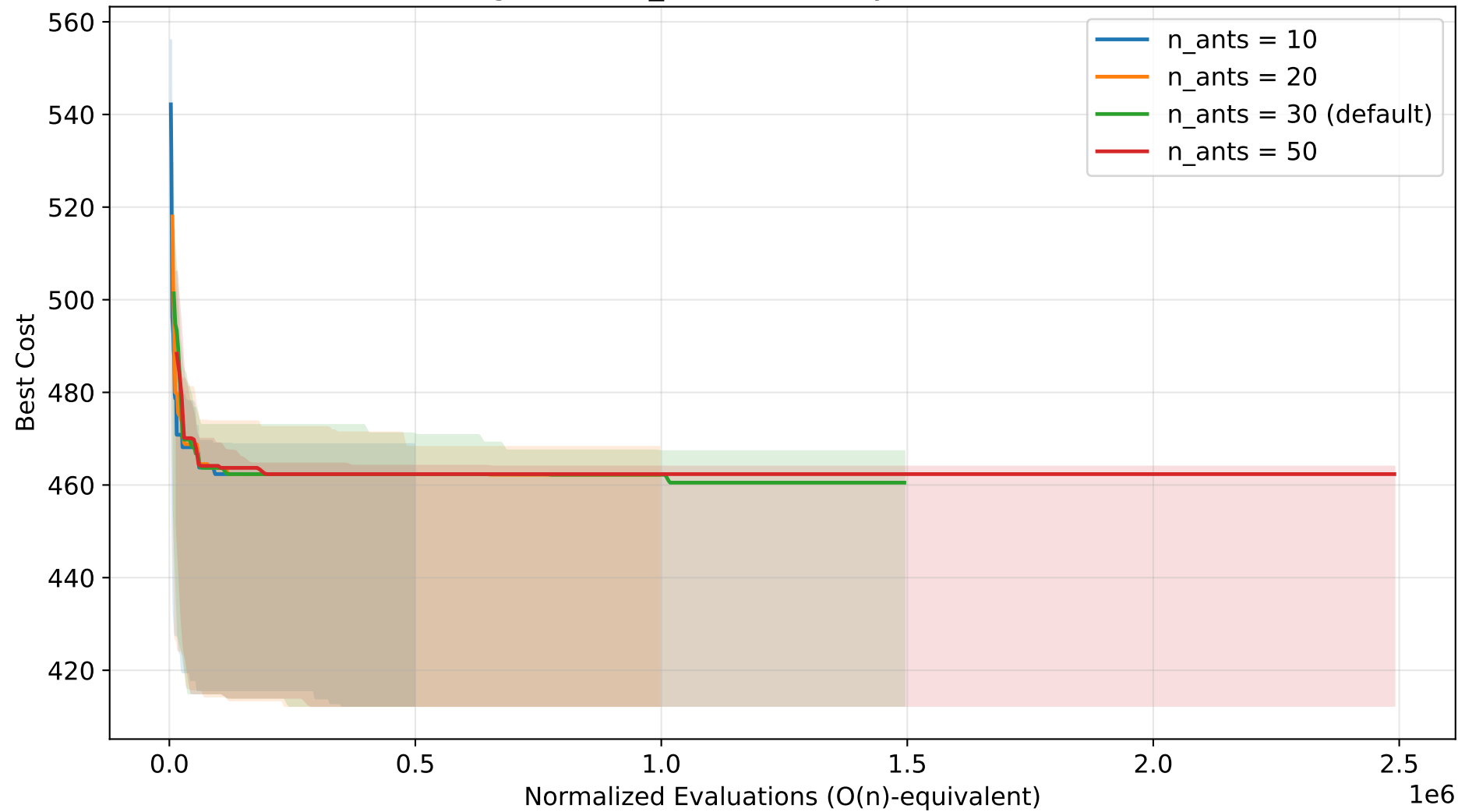
ACO Convergence — n_ants sensitivity (TSP n=30, normalized)
