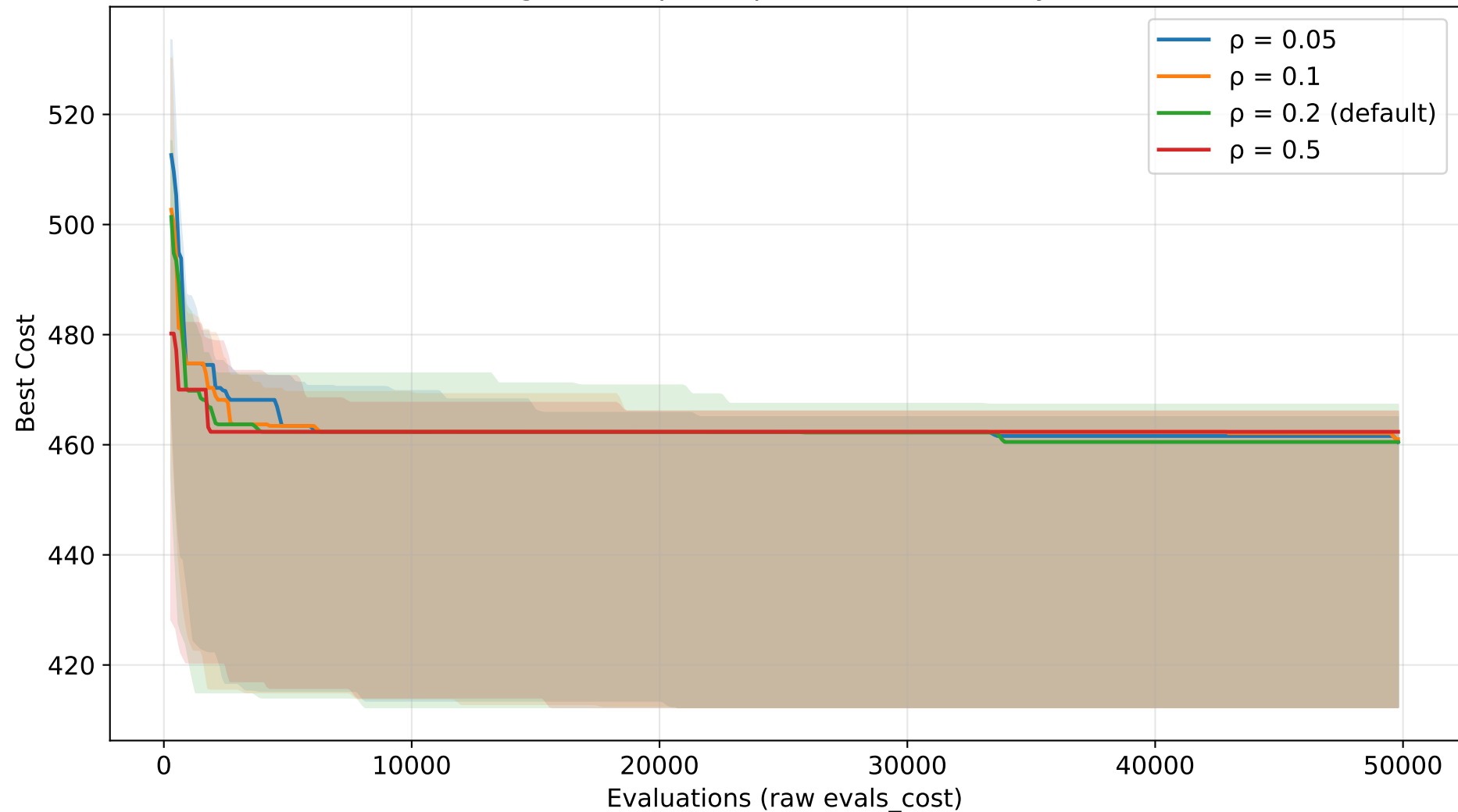
ACO Convergence — \rho (evaporation) sensitivity (TSP n=30)
