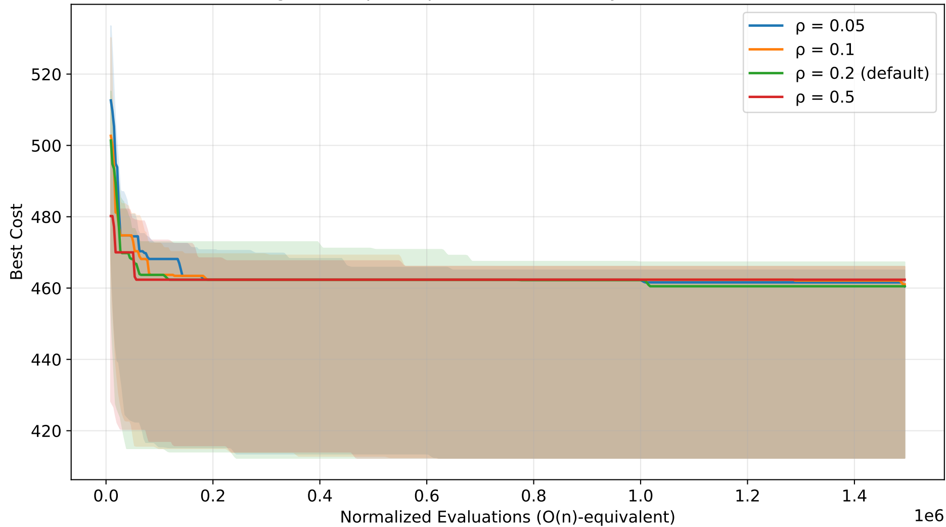
ACO Convergence — \rho (evaporation) sensitivity (TSP n=30, normalized)
