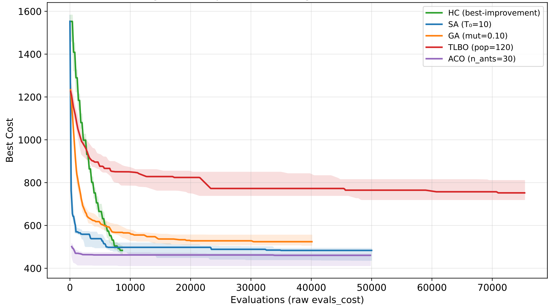
Convergence Comparison — All Algorithms (TSP n=30, raw evals)
