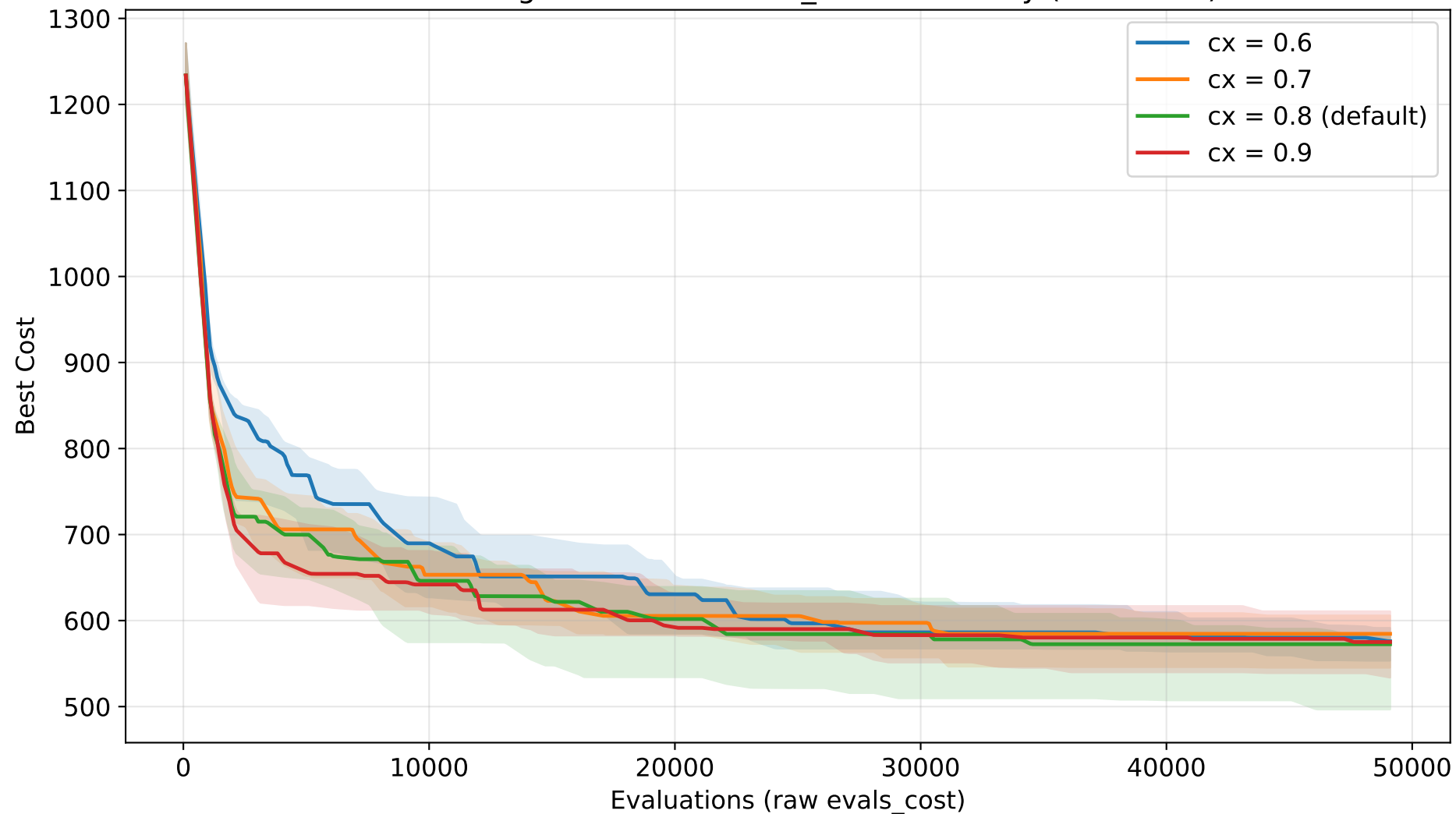
GA Convergence — crossover_rate sensitivity (TSP n=30)
