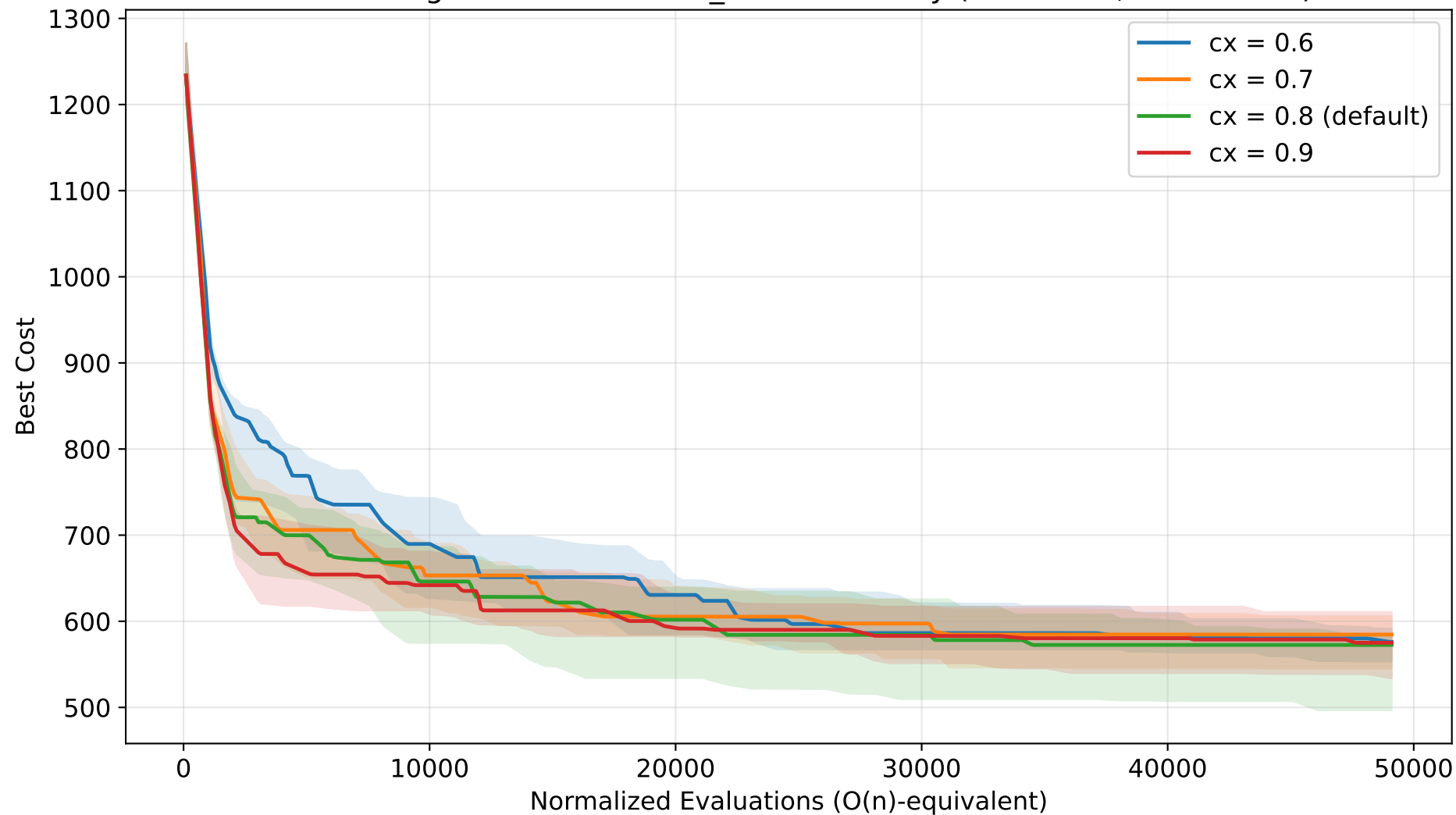
GA Convergence — crossover_rate sensitivity (TSP n=30, normalized)
