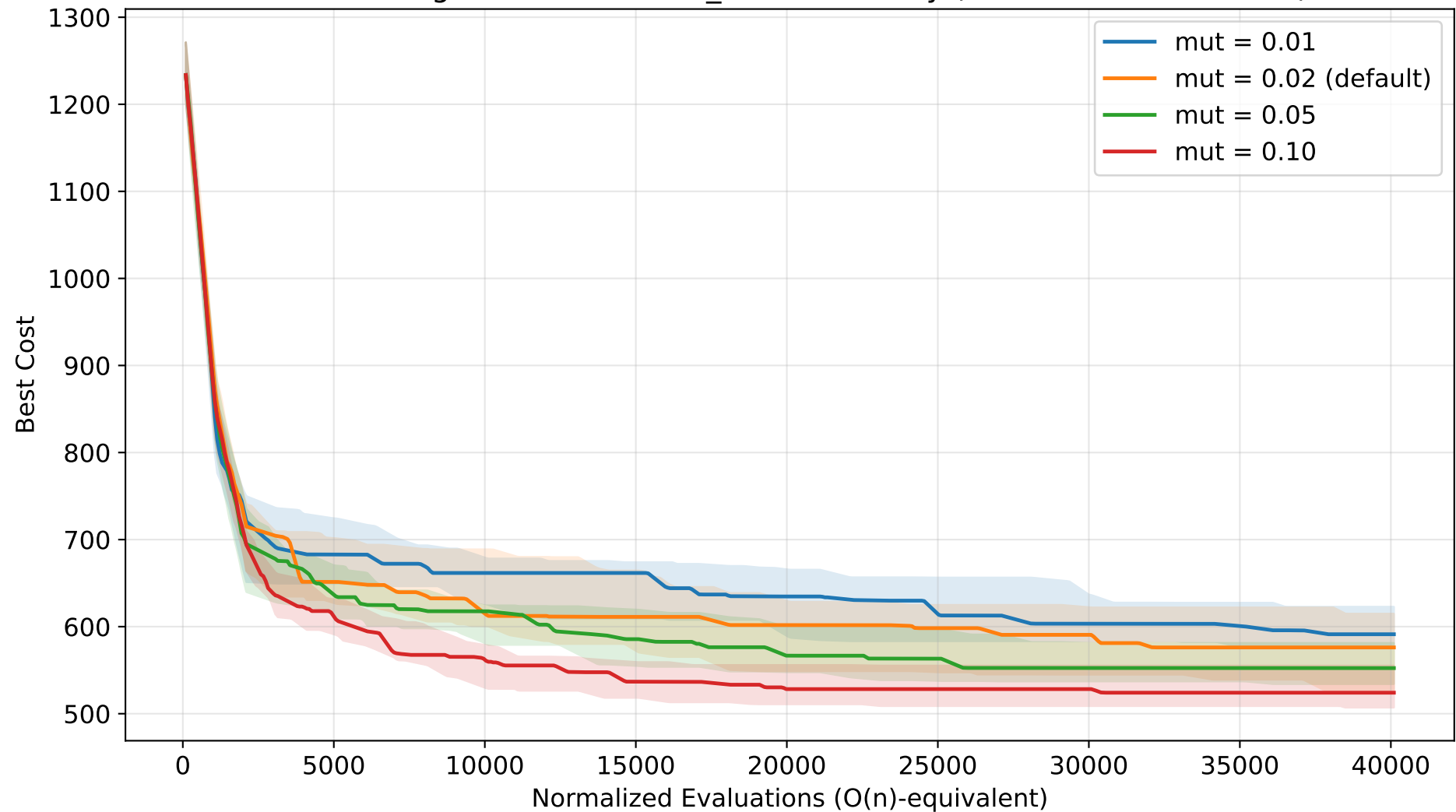
GA Convergence — mutation_rate sensitivity (TSP n=30, normalized)
