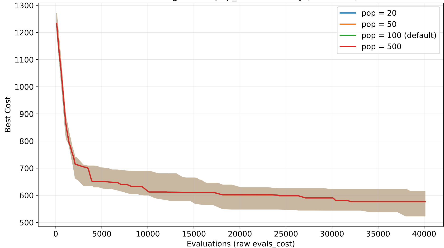
GA Convergence — pop_size sensitivity (TSP n=30)
