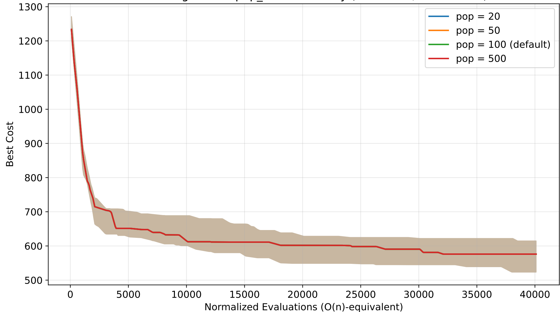
GA Convergence — pop_size sensitivity (TSP n=30, normalized)
