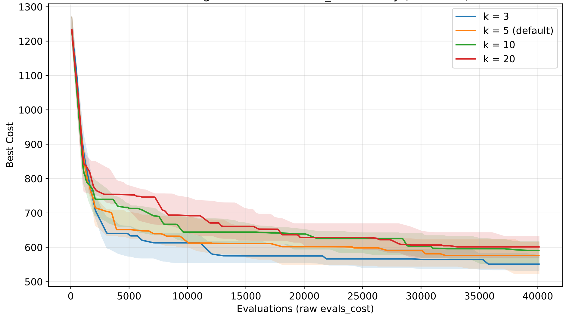
GA Convergence — tournament_k sensitivity (TSP n=30)
