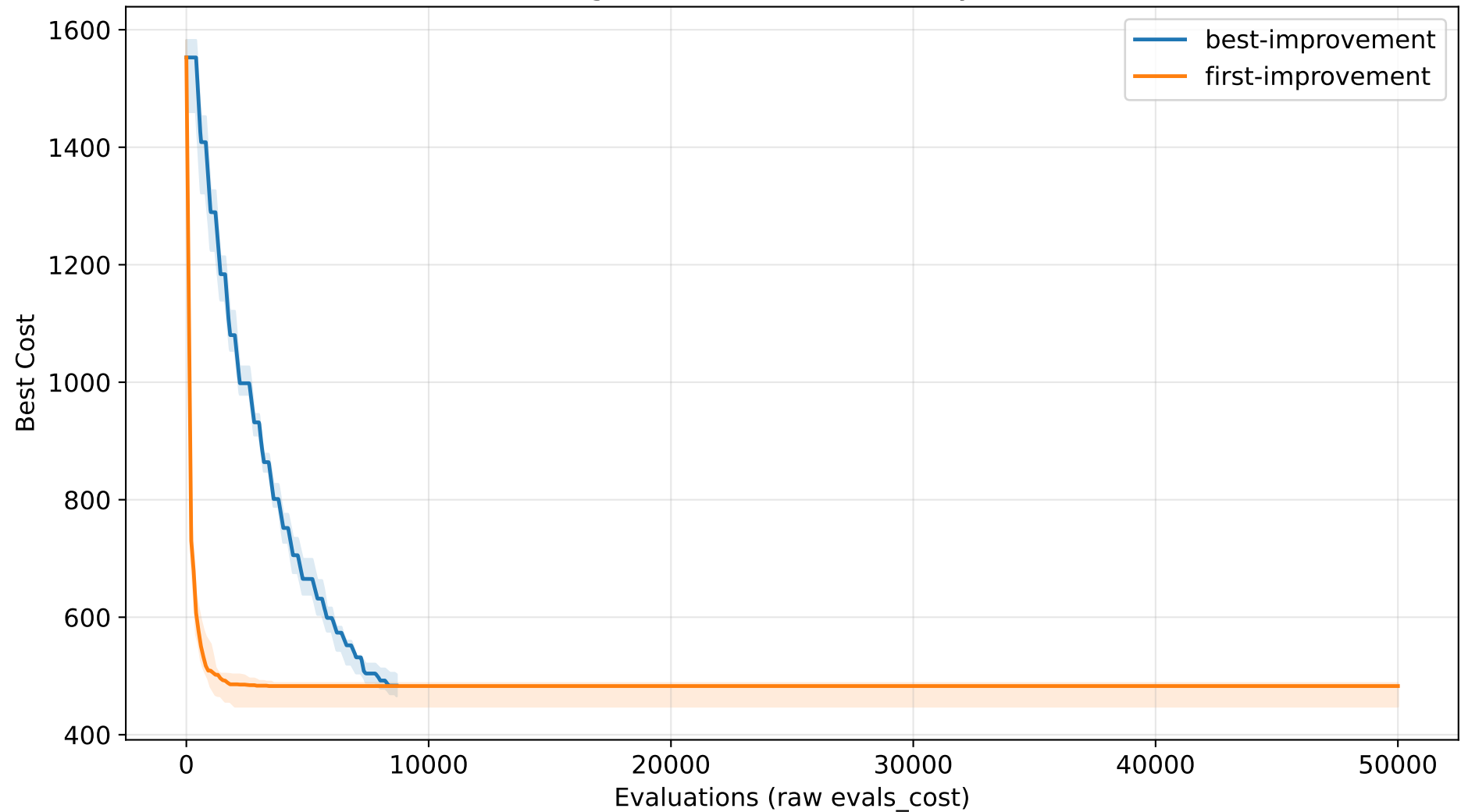
HC Convergence — mode sensitivity (TSP n=30)
