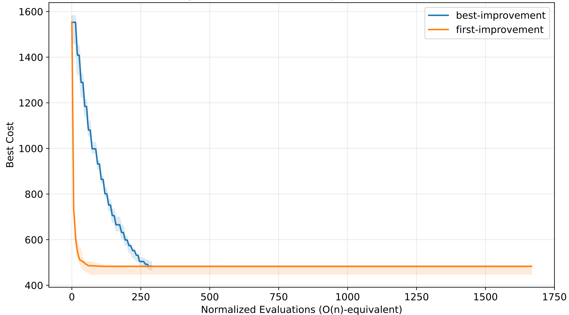
HC Convergence — mode sensitivity (TSP n=30, normalized)
