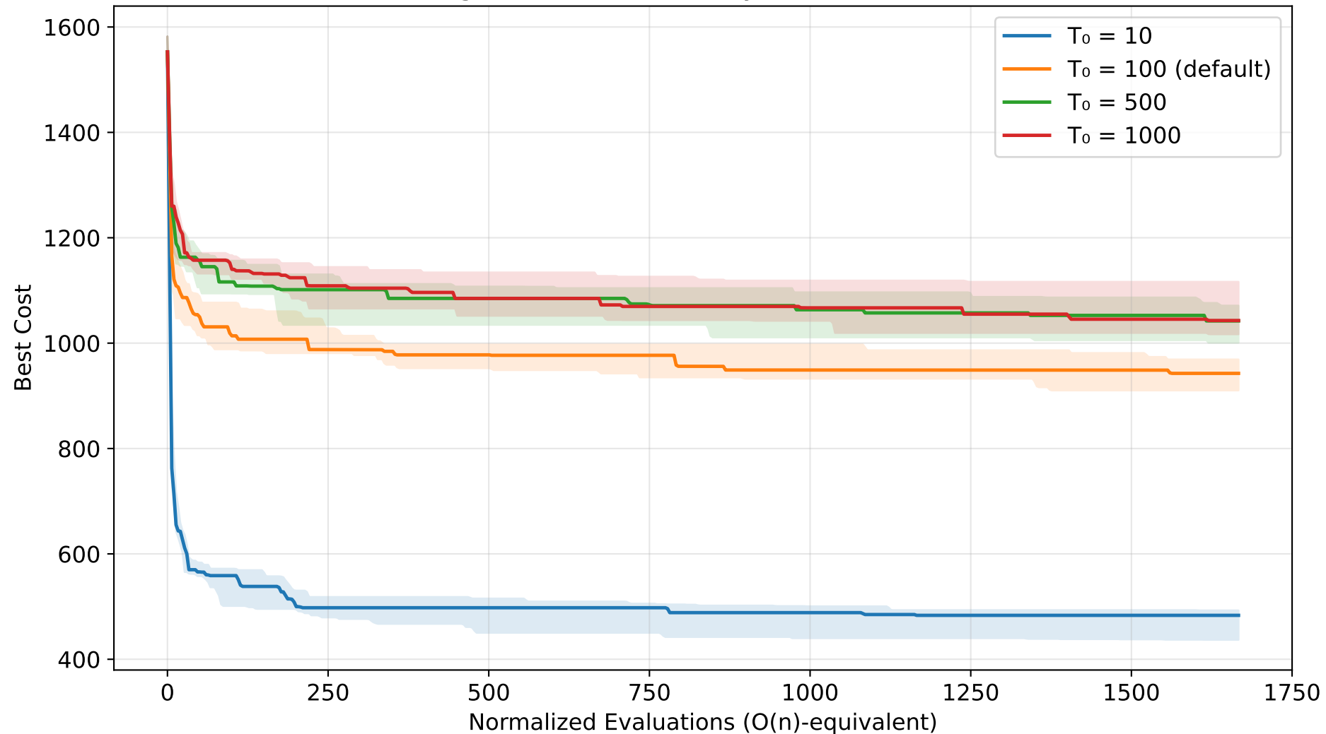
SA Convergence — T_0 sensitivity (TSP n=30 , normalized)
