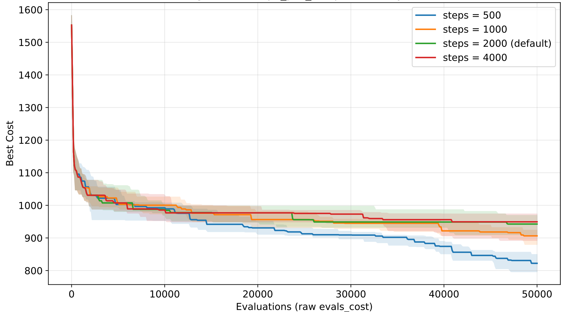
SA Convergence — steps_per_temp sensitivity (TSP n=30)
