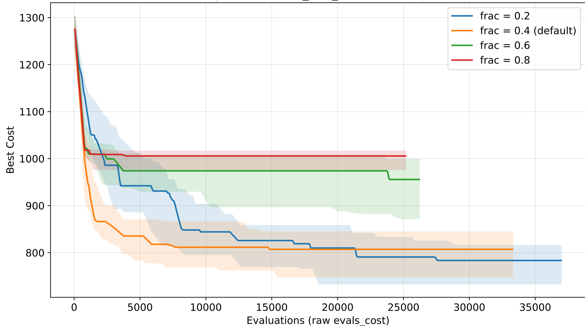
TLBO Convergence — move_frac_max sensitivity (TSP n=30)
