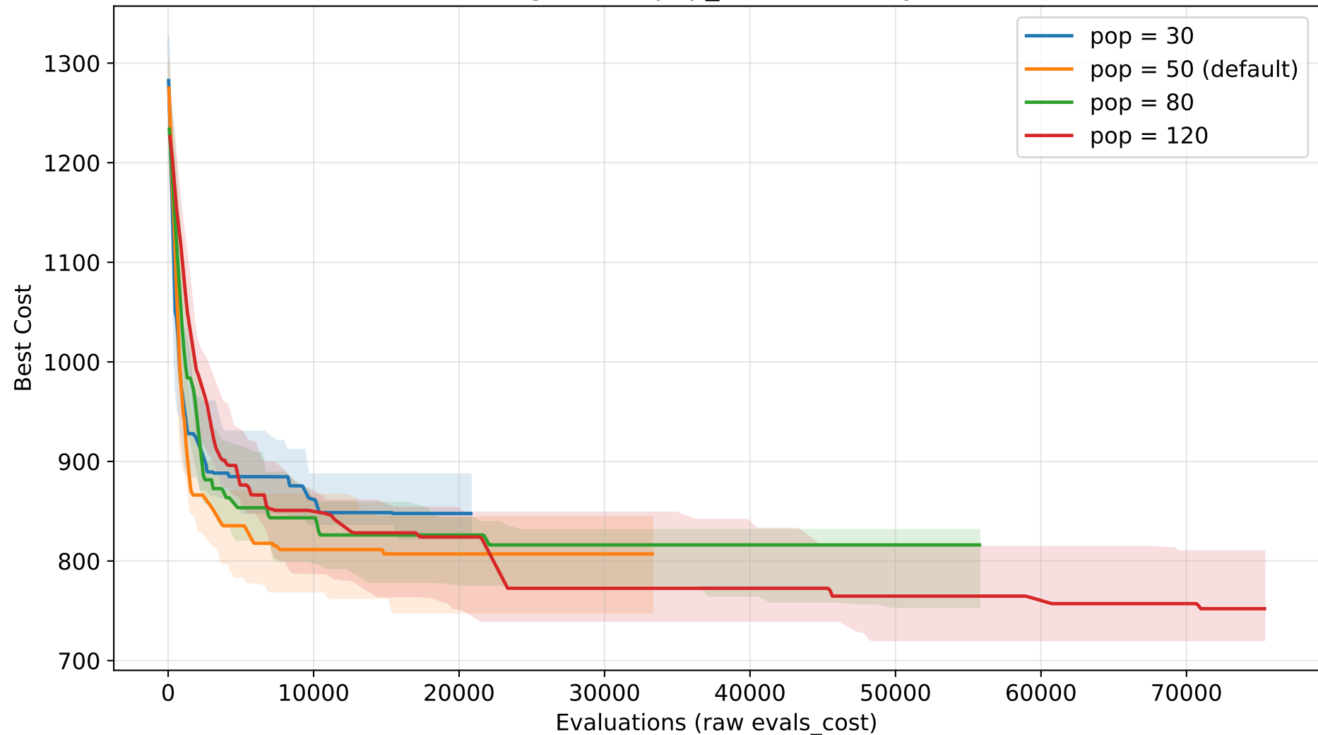
TLBO Convergence — pop_size sensitivity (TSP n=30)
