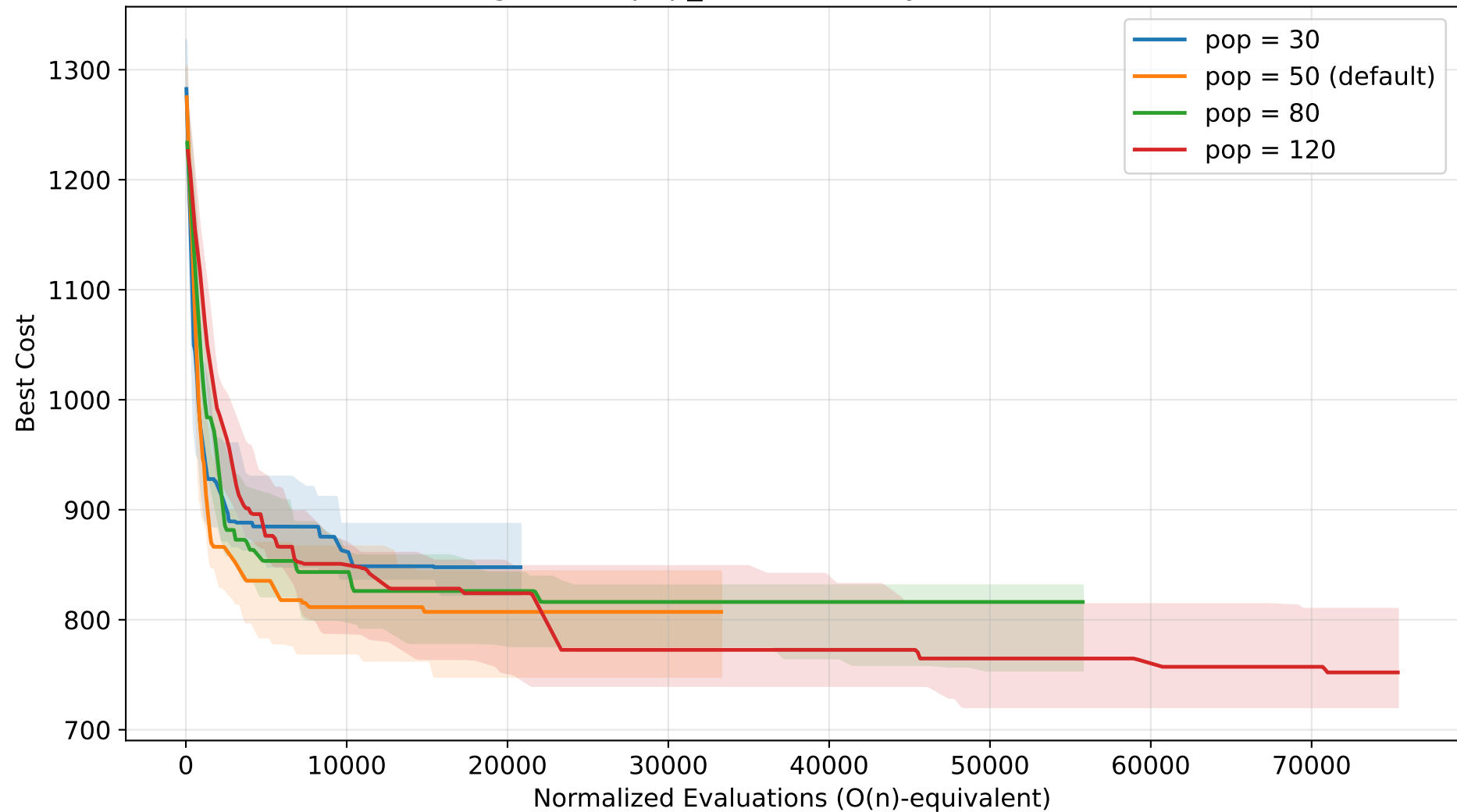
TLBO Convergence — pop_size sensitivity (TSP n=30, normalized)
