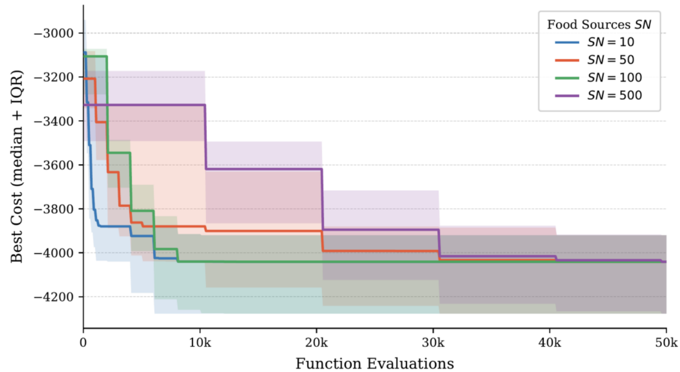
ABC Parameter Sensitivity — Food Sources SN Knapsack (step-wise best-so-far, median + IQR)
