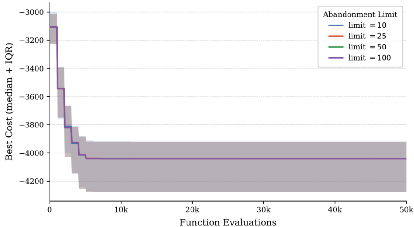
ABC Parameter Sensitivity — Abandonment Limit Knapsack (step-wise best-so-far, median + IQR)
